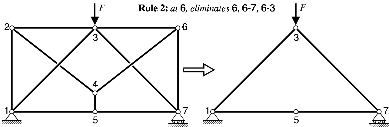
Fig 3. Example of simplification rules and their application to a simple truss (adapted from [3]).
