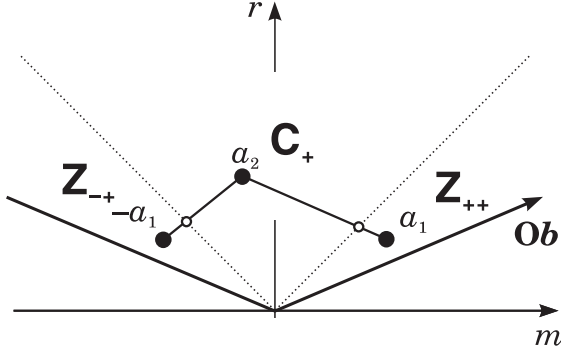
Figure III.67d: (cont.) Enumeration of basic two-dimensional types (the last part: the types NZ , NC , and ZC ).
