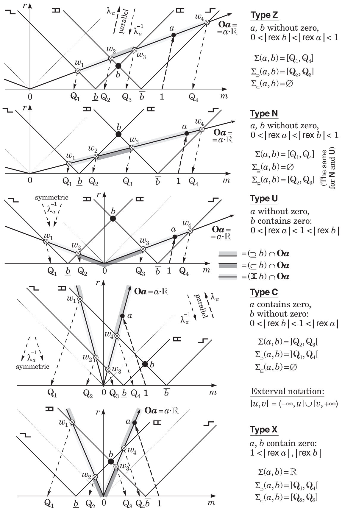
Figure III.47: Diagrammatic solutions of the a \cdot x \diamond b relation: regular cases (types Z , N , and U ), and singular cases (types C and X ).
