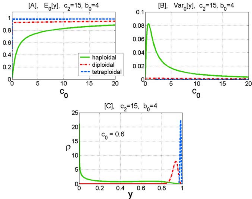
Fig. 5. Color online: Mode \{AAB\} : c_2 = 15 , b_0 = 4 ; Panels A: mean per copy E_0(y)(c_0) and B: variance per copy Var_0(y)(c_0) . Panel C: protein distributions \rho(y) for the haploid, diploid, tetraploid systems for c_0 = 0.6 (at which haploid system has \max[Var_0(y)(c_0)] ).
