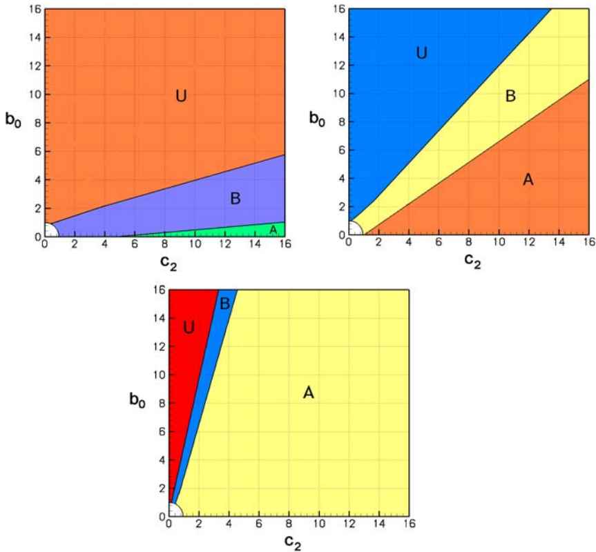
Fig. 3. Color online: Three regions in (c_2, b_0) plane corresponding to three modes of gene activation \{A\}, \{B\}, \{U\} . Panel A: the haploid gene, Panel B: the diploid gene and Panel C: the tetraploid gene.
