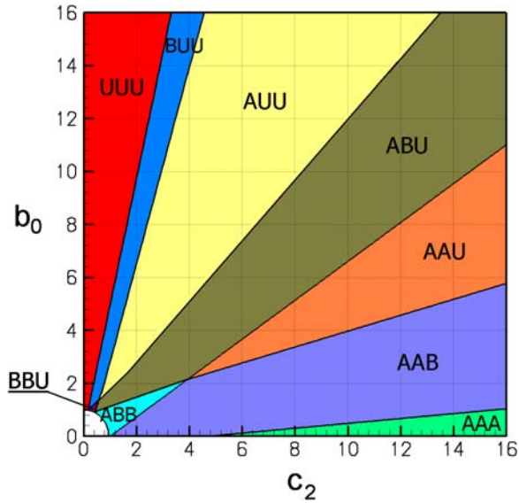
Fig. 4. Color online: Nine modes of synergistic gene activation; The notation is such that: {ABU} denotes that the tetraploid gene is in the {A} mode, the diploid gene is in the {B} mode and the haploid gene is in the {U} mode. The activation profiles for three marked points in (c_2, b_0) plane are analyzed in Figs. 5, 6 and 7.
