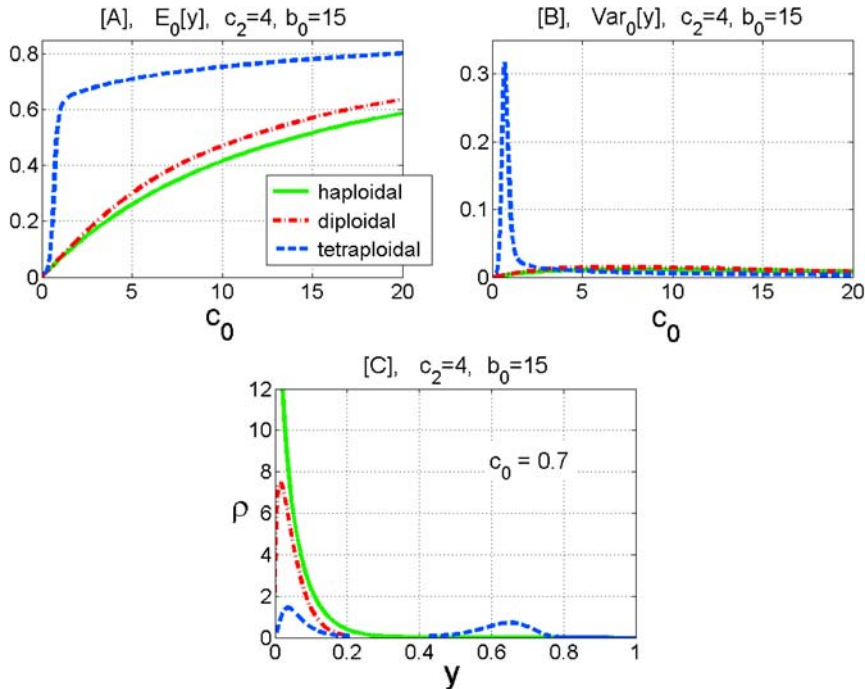
Fig. 7. Color online: Mode \{BUU\} : c_2 = 4 , b_0 = 15 ; Panels A: mean per copy E_0(y)(c_0) and B: variance per copy Var_0(y)(c_0) . Panel C protein distributions \rho(y) for haploid, diploid, tetraploid systems for c_0 = 0.7 (at which tetraploid system has \max[Var_0(y)(c_0)] ).
