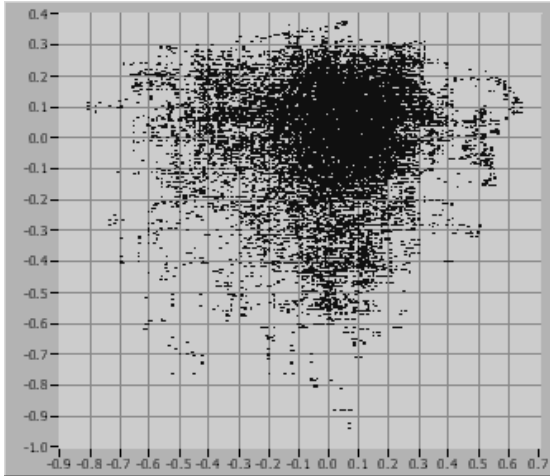
Fig. 7. The NSP pattern from Fig. 6b after median filtering (filter order k = 5 ) (after Ref. 1)
