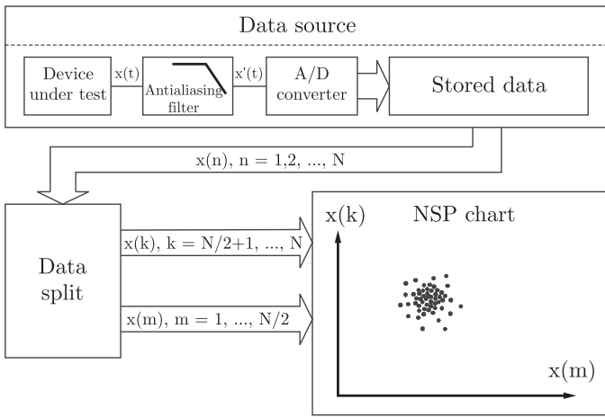
Fig. 2. Schematic diagram of the measurement system based on the NSP method; x(t) – noise signal, x'(t) – noise signal after antialiasing (lowpass) filtration, x(n) – stored data, x(k) , x(m) – subsequences after splitting sequence x(n)
