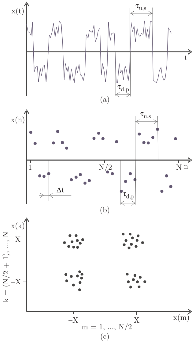
Fig. 5. Illustration of results of the NSP method for a noise signal containing Gaussian noise and RTS noise: (a) – noise signal, (b) – sampled signal data, (c) – data in XY plane
