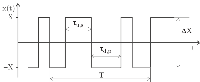
Fig. 1. Typical two-level RTS noise \tau_{u,s} – the s -th duration of an impulse in the up time, \tau_{d,p} – the p -th duration of an impulse in the down time, \Delta X – the amplitude of RTS noise, T – observation time
