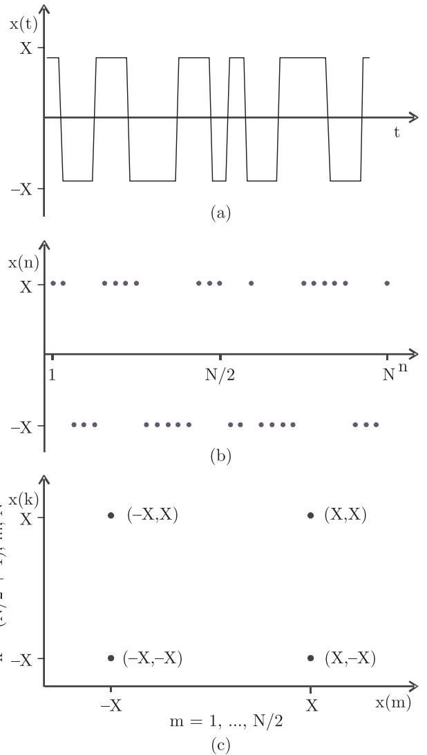
Fig. 4. Illustration of the idea of the NSP method for inherent noise signal which contains only RTS noise: (a) – noise signal, (b) – sampled signal data, (c) – data in XY plane
