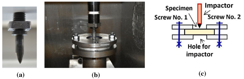
Fig. 1 Details of the loading chain of testing stand: a general view of the impactor; b specimen mounted in the machine grips; c scheme of impact of the target-plate
