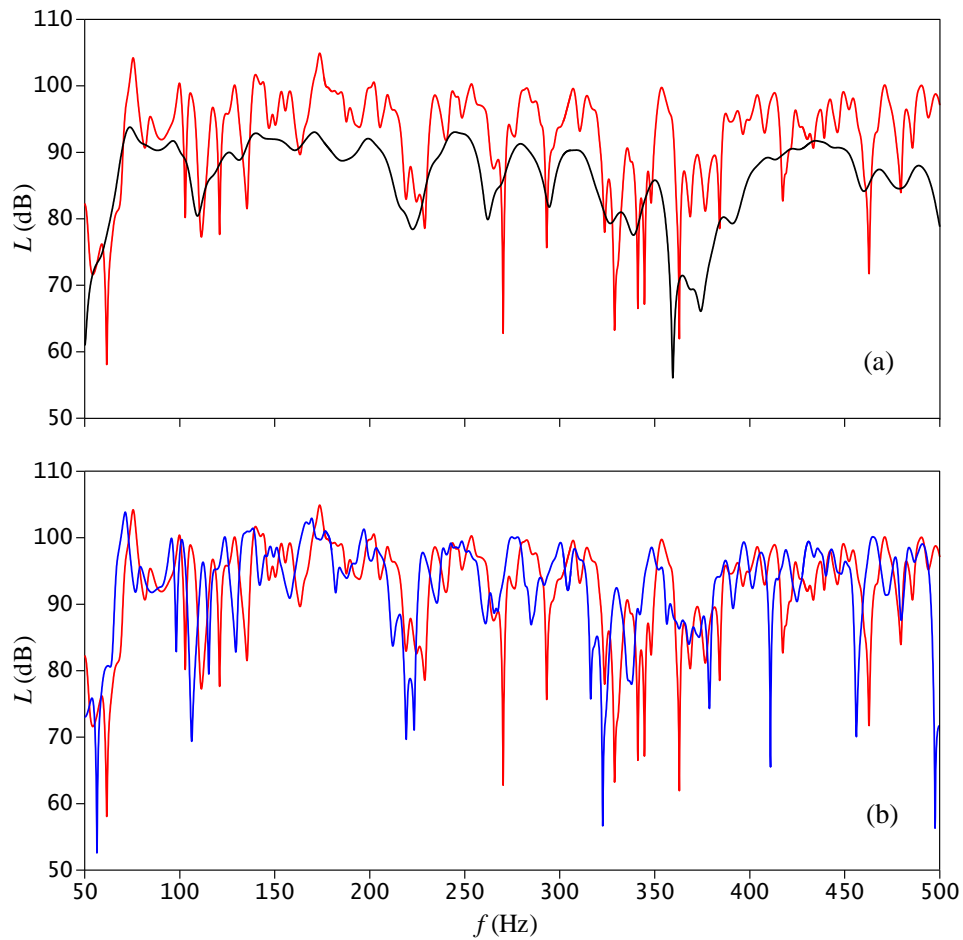
Figure 2. Comparison of the room transfer functions predicted at the observation point: x = 2 m, y = 3 m, z = 1.2 m, for wall impedances: \zeta = 10 (black line), \zeta = 10 + j15 (red line), \zeta = 10 - j15 (blue line)
