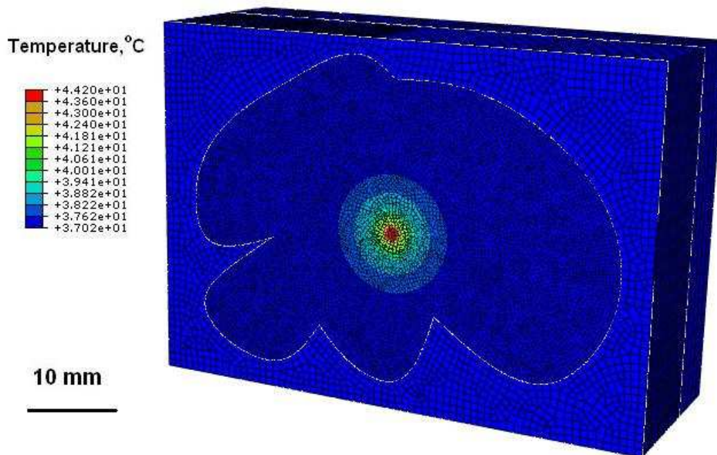
Fig. 10 Temperature pattern in the rat liver across the acoustic beam axis at the axial distance 21 mm from transducer
