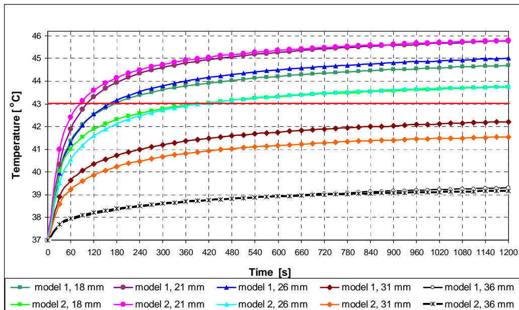
Fig. 6. Comparison of the temperature variation in time predicted by numerical calculation, for Models 1 and 2, at different distances from the transducer
