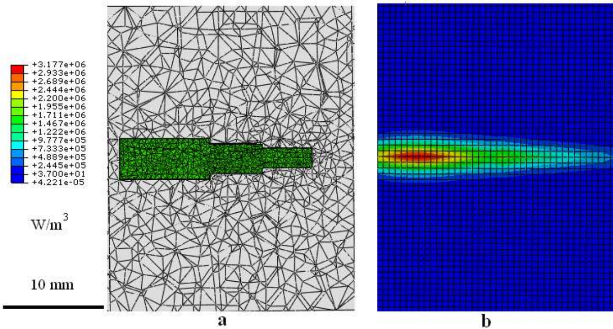
Fig. 4. Distribution of power of heat sources density: a) Model 1, b) Model 2
