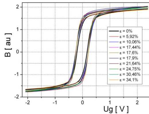
Fig. 7. Magnetic hysteresis loops of undamaged and damaged specimens due to creep of the 13HMF steel.
