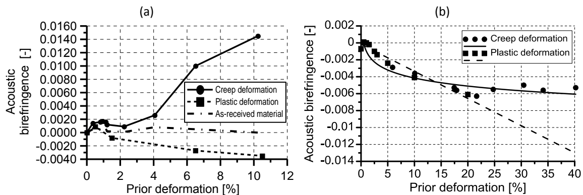
Fig. 5. Acoustic birefringence B variations due to prior deformation for: (a) 40HNMA steel; (b) 13HMF steel.
