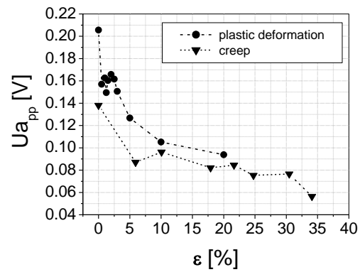
Fig. 9. Dependence between amplitudes of Ua envelopes and prior deformation due to plastic flow (circles) and creep (triangles).
