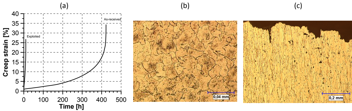
Fig. 1. Comparison of tensile creep curves ( \sigma=230 MPa, T=773 K) for the 13HMF steel in the as-received state and after exploitation by a period of 144000 h (a), and its metallographic structures for the initial state (b) and after 144000 h of work (c).
