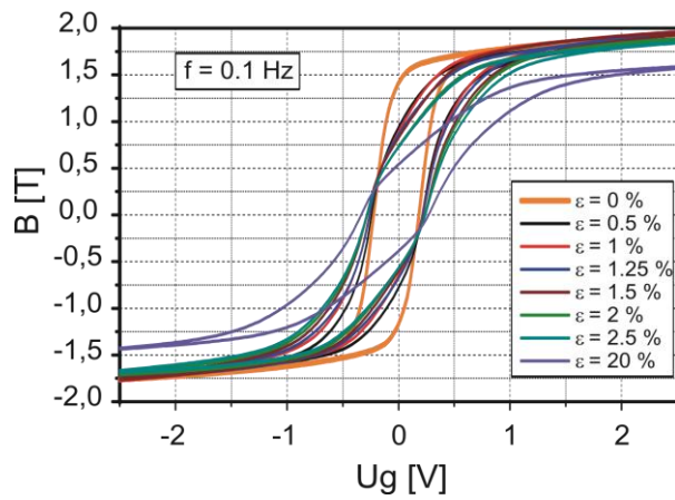
Fig. 6. Magnetic hysteresis loops of undamaged and damaged specimens due to plastic flow of the 13HMF steel.
