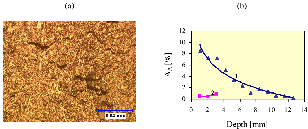
Fig. 10. Microstructural observations of the 40HNMA: (a) strong damage close to fracture surface, magnification 500x; (b) changes of the void area fractions ( A_A [%]) as a function of distance from the fracture surface for 40HNMA steel deformed due to: (1) creep up to 6.5%; (2) plastic flow up to fracture (19%).
