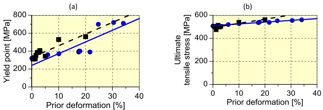
Fig. 4. Variation of tensile parameters of the 13HMF steel due to creep (solid lines) and plastic (broken lines) deformations: (a) yield point; (b) ultimate tensile stress.
