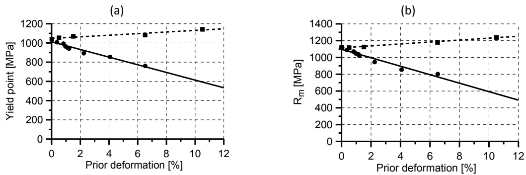
Fig. 3. Variation of the tensile parameters for the 40HMNA steel due to creep (solid lines) and plastic (broken lines) deformations: (a) yield point; (b) ultimate tensile stress.
