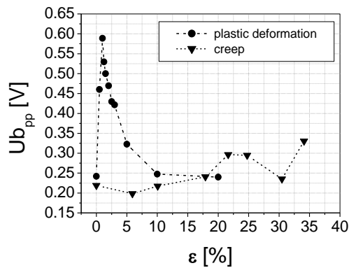
Fig. 8. Dependence between the amplitudes of Ub envelopes and deformation for specimens after plastic flow (circles) and after creep (triangles).
