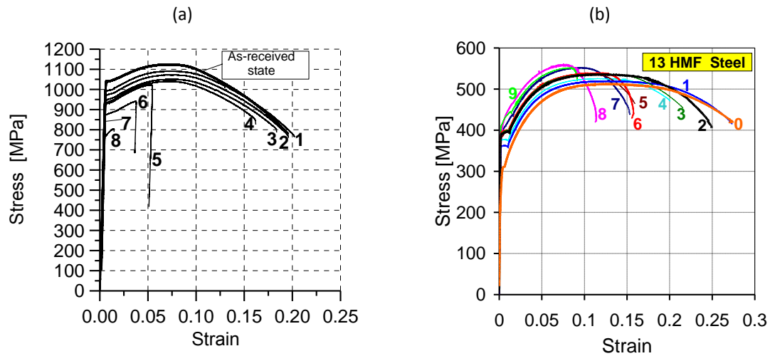
Fig. 2. Tension characteristics of: (a) the 40HMNA steel after creep for 100h (1), 241h (2), 360h (3), 452h (4), 550h (5), 792h (6), 929h (7) and 988h (8), and (b) the 13HMF steel after creep for 149h (1), 300h (2), 360h (3), 407h (4), 441h (5), 587h (6), 664h (7), 796h (8) and 1720h (9).
