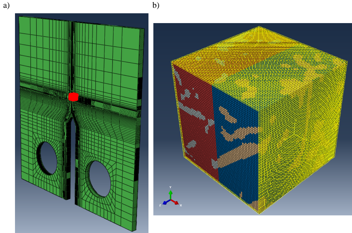
Figure 6.42. The FEM model for C-T test with account of real IPC microstructure developed in ABAQUS (a) outer, global model of C-T specimen with effective elastic properties, node set from which displacements are taken for the submodel marked in red, (b) submodel of real \text{Al}_2\text{O}_3/\text{Cu} IPC microstructure obtained with micro-CT imaging (displacement boundary conditions marked in yellow).
