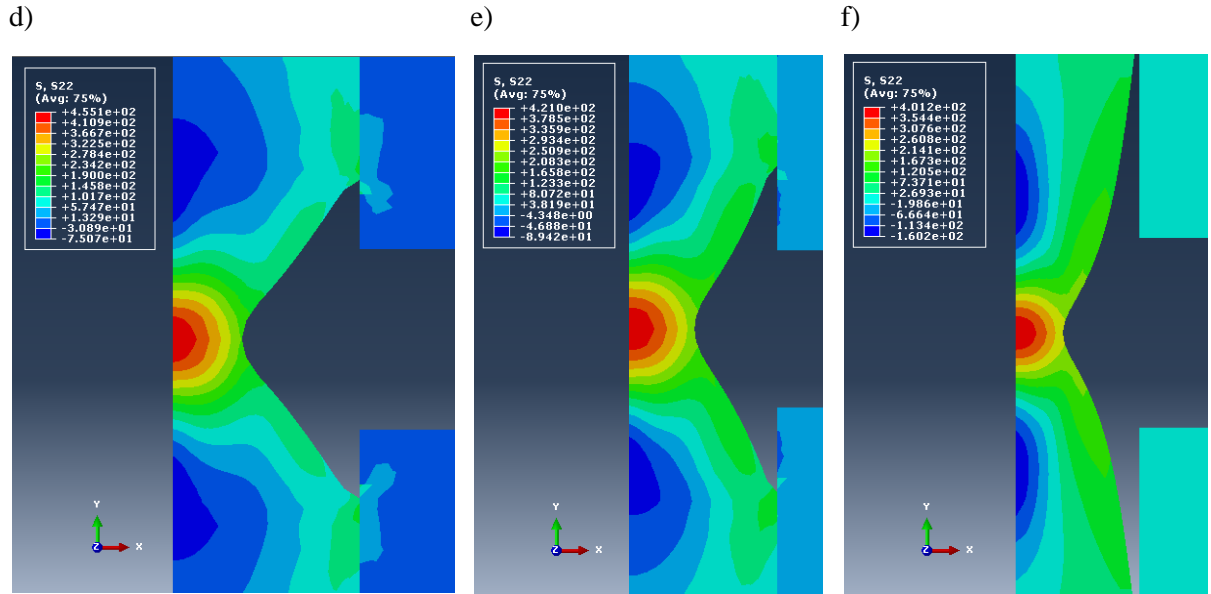
Figure 6.15. Axisymmetric model of uniaxial tension of cracked elastic matrix with reinforcing elastic-plastic fibre at fixed debonding lengths. ABAQUS results: (a-c) for \text{Al}_2\text{O}_3/\text{Al} , (d-f) for \text{Al}_2\text{O}_3/\text{Cu} , at loadings u_2 : (d) 0.16 mm, (e) 0.175 mm, (f) 0.2 mm. Distributions of axial stresses \sigma_{22} : (a, d) \psi=0.4 , (b, e) \psi=0.6 , (c, f) \psi=2.0 (images not in the same scale)
