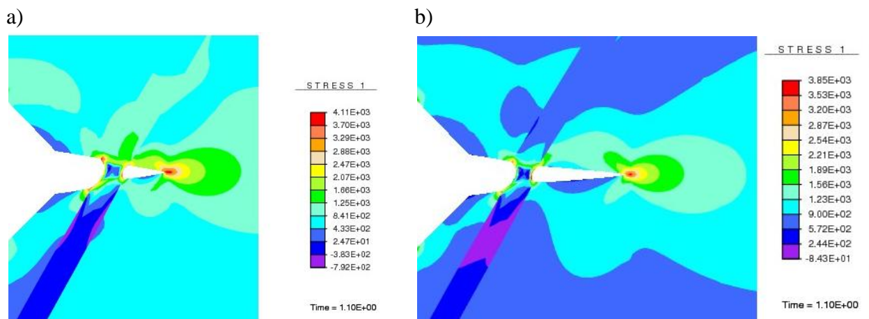
Figure 6.29. Horizontal stress distributions for fibre inclined at 60° to the crack plane for: (a) initial and (b) increased crack length .
