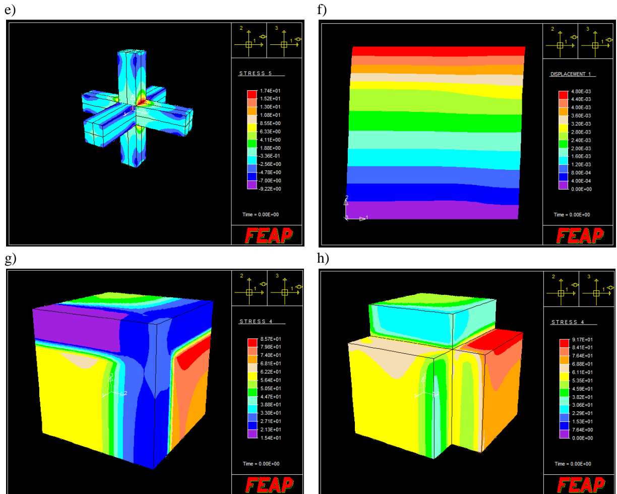
Figure 5.10. Sample results of the calculations for the 3D cross FEM model in FEAP 7.5, (a–e) uniaxial tension, 0.93 of metal volume fraction, (f–h) simple shear, 0.16 of metal volume fraction: a) distribution of displacements in loading direction u_1 , showed in deformed state enlarged 100 \times , (b, c) distributions of normal stresses in loading direction \sigma_{11} , (d, e) distributions of shear stresses in loading direction \tau_{23} , f) distribution of displacements in loading direction u_1 , showed in deformed state enlarged 100 \times , (g, h) distributions of shear stresses in direction perpendicular to loading \tau_{12} .
