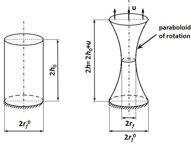
Figure 3.3. Geometry of the necking ligament in the model of Mataga (1989).
