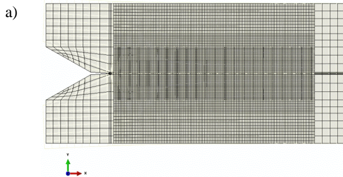
Figure 6.35. Detailed view of the crack tip neighbourhood with family of parallel reinforcing fibres.
