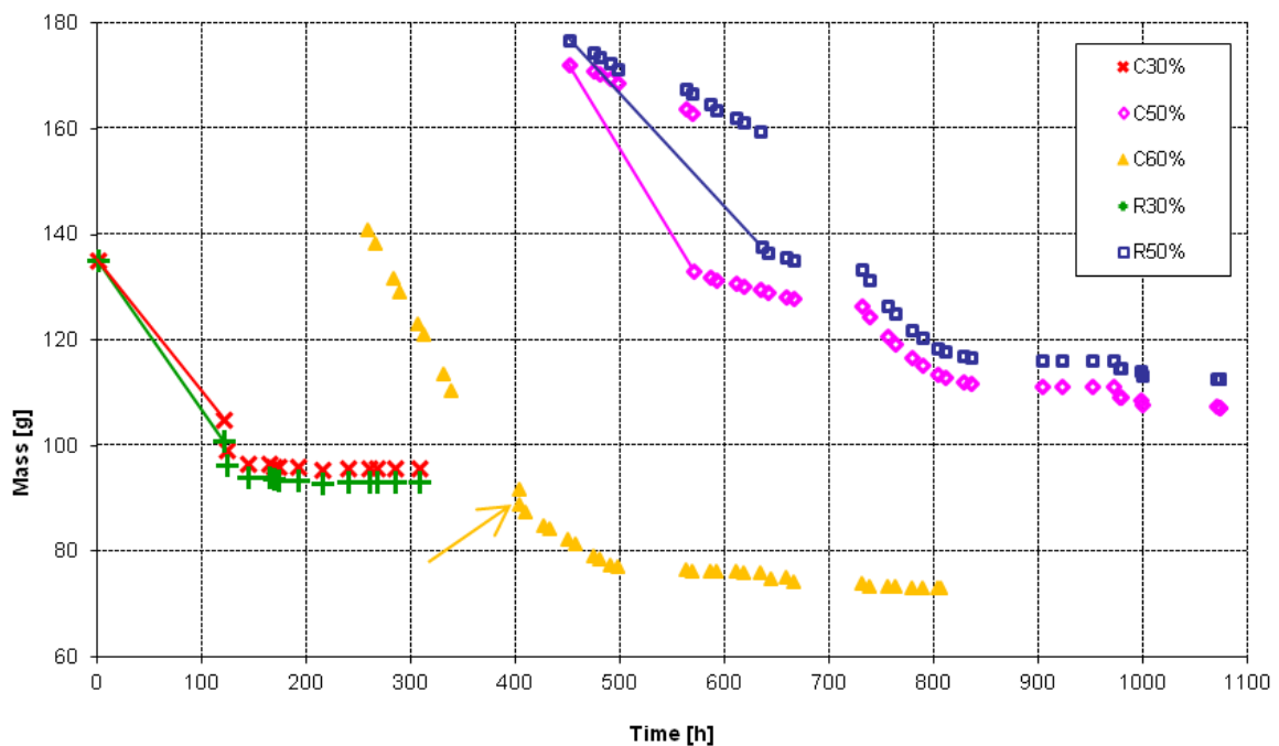
Figure A2. Drying curves for green alumina-PFA samples. Except for C60% sample, all curves start at the moment of casting the slurries into forms. The lines connect these points with points after removing samples from frames, from where the direct mass of the sample was measured. Arrow indicates point after removing the sample C60% from frames, as it was not possible for this sample to indicate the value of the mass of just poured slurry.
