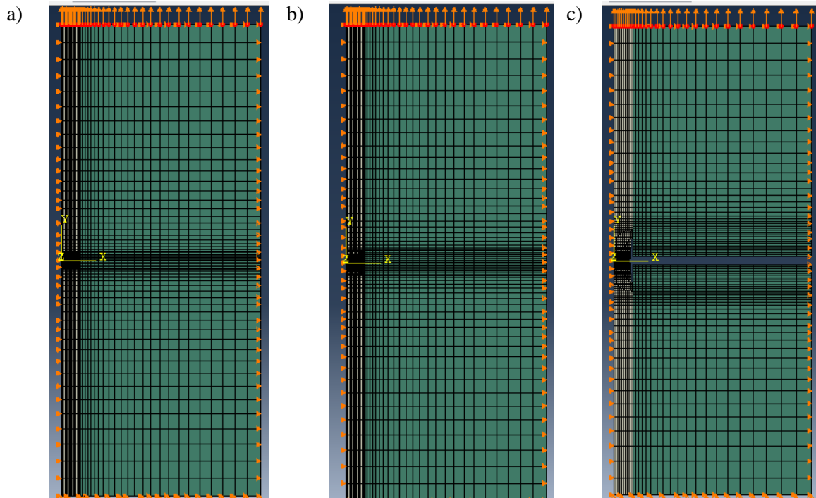
Figure 6.14. FEM model (FEM mesh created with FEAP); displacement loading and boundary conditions for three values of nondimensional debonding parameter \psi : a) \psi=0.4 , b) \psi=0.6 and c) \psi=2.0
