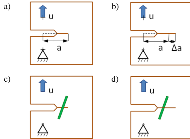
Figure 6.26. Scheme of C-T test to determine energy release rate and fracture toughness increase due to bridging: (a), (b) specimens from monolithic ceramic material, (c), (d) ceramic specimens with metallic reinforcements; (a), (c) – initial state, (b), (d) – state at infinitesimally increased crack length.
