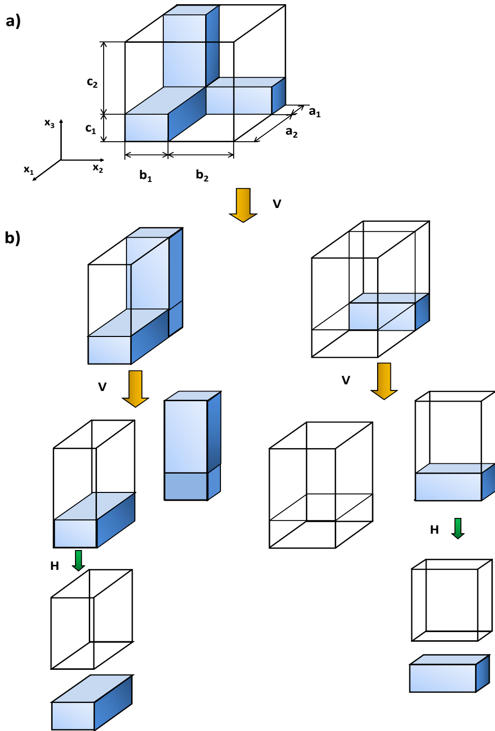
Figure 2.3 (a) Feng et al. (2003, 2004) unit cell of an interpenetrating two-phase composite model and (b) its vertical (V) and horizontal (H) decomposition (based on Feng et al. (2003, 2004), with the permission of publishers).
