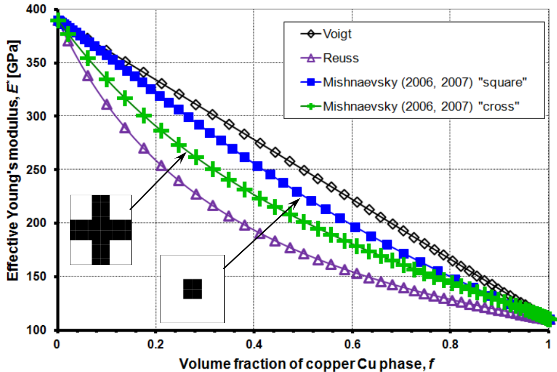
Figure 5.8. Influence of the model microstructure on the effective Young's modulus of \text{Al}_2\text{O}_3/\text{Cu} composite: the results of Mishnaevsky (2006, 2007b) procedure implemented for two different microstructures – “cross” microstructure and matrix – inclusion “square” microstructure (reproduced from Poniznik et al. (2008) with permission of the publisher)
