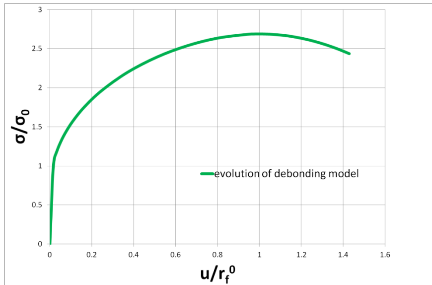
Figure 6.24. Stress-displacement relationship in the reinforcing fibre obtained with the FEM model accounting for the fibre/matrix debonding evolution.
