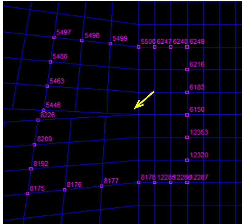
Figure 6.28. Nodes forming the 3 rd contour for the J -integral (yellow arrow indicates crack tip)
