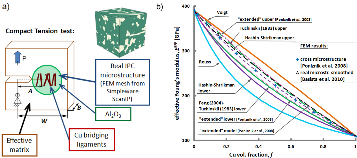
Figure 6.38. Scheme of the Compact-Tension test model of the IPC with real material microstructure obtained from micro-CT: (a) FE mesh in the vicinity of the crack based on the micro-CT data, (b) analytical and numerical models for effective elastic properties used for the remaining part of the C-T specimen (based on Poniznik et al. , 2008, Basista et al. , 2010 and Basista et al. , 2016, with the permission of publishers).
