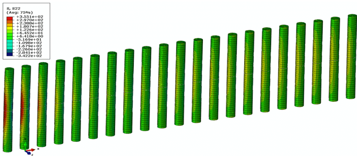
Figure 6.37. Numerical model and results from ABAQUS: a) vertical logarithmic strain distribution in reinforcing fibres, b) vertical stress distribution in reinforcing fibres.
