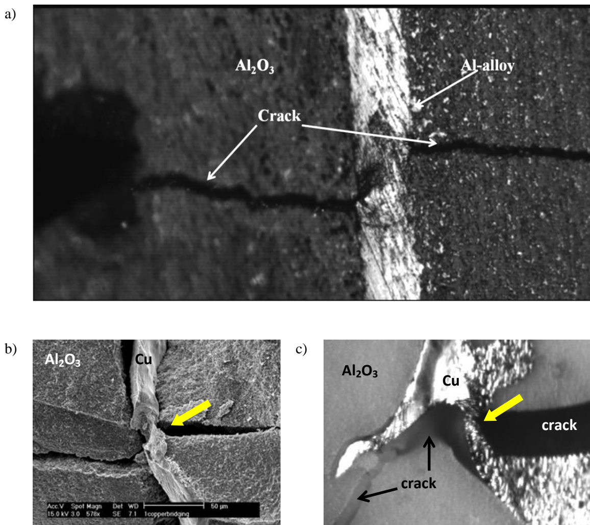
Figure 3.2. Crack bridging by metal ligament undergoing plastic deformation and decohesion from the surrounding ceramic matrix; (a) \text{Al}_2\text{O}_3/\text{Al} infiltrated composite (courtesy of PZMK IPPT PAN); (b) \text{Al}_2\text{O}_3/\text{Cu} infiltrated composite (reproduced from Poniznik et al. 2015 with permission of Int. J. Damage Mechanics ); (c) \text{Al}_2\text{O}_3/\text{Cu} infiltrated composite.
