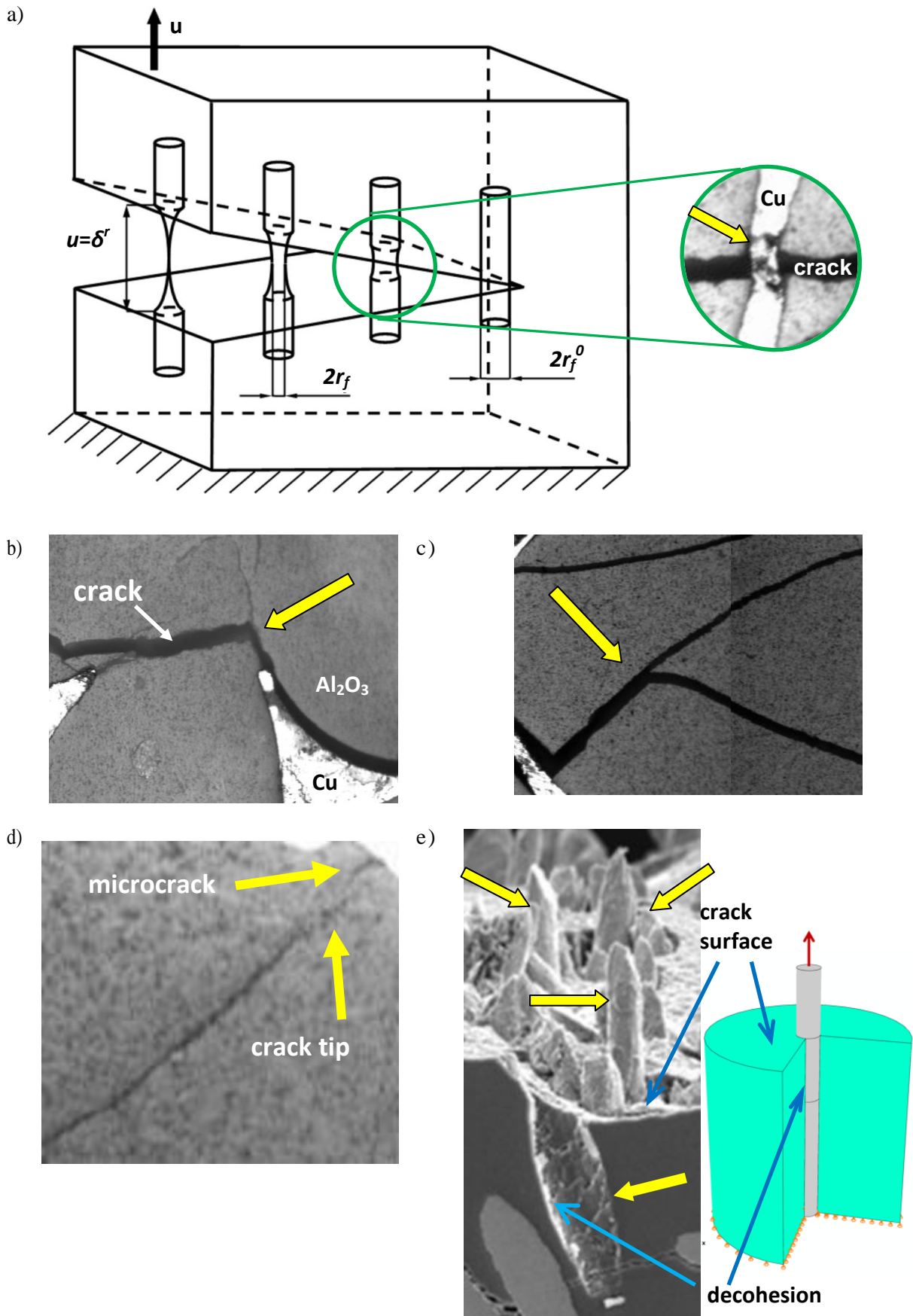
Figure 3.1. Schemes of crack toughening mechanisms in metal-ceramic composites (yellow arrows mark respective physical mechanisms); (a) crack bridging (reproduced from Ponižnik et al. , 2015 with
