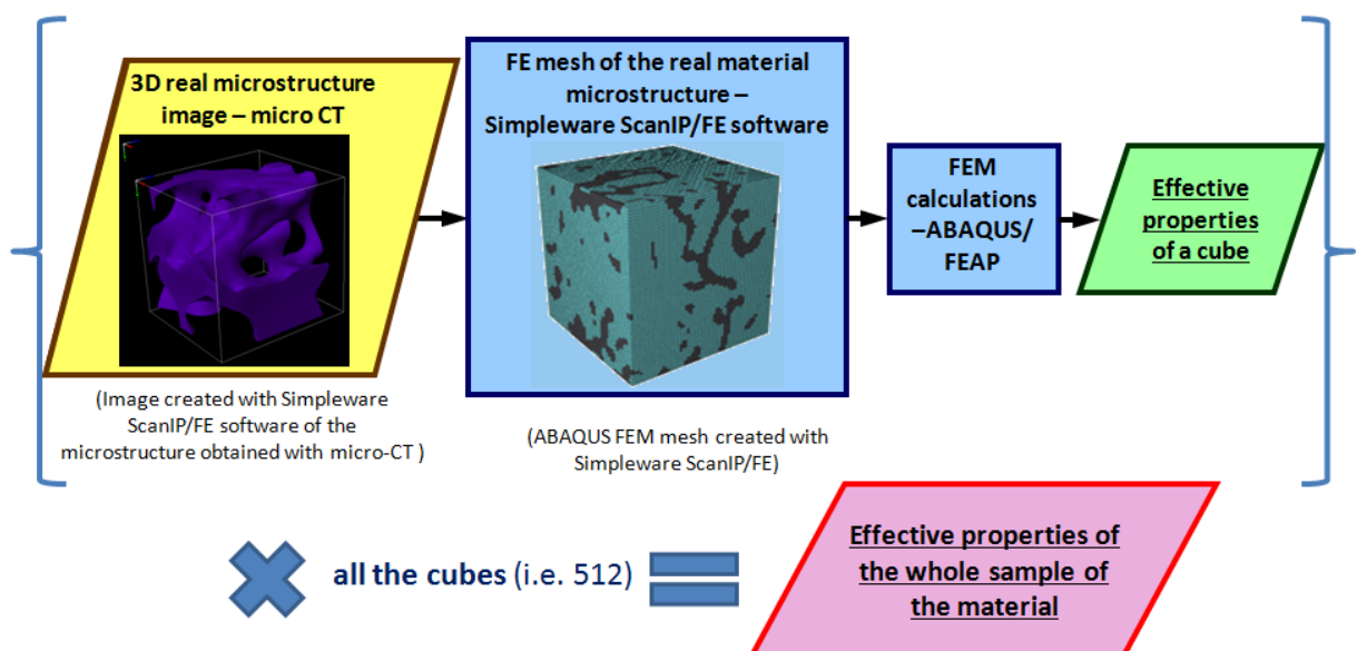
Figure 5.11. Scheme of the numerical approach used for the real composite microstructures.
