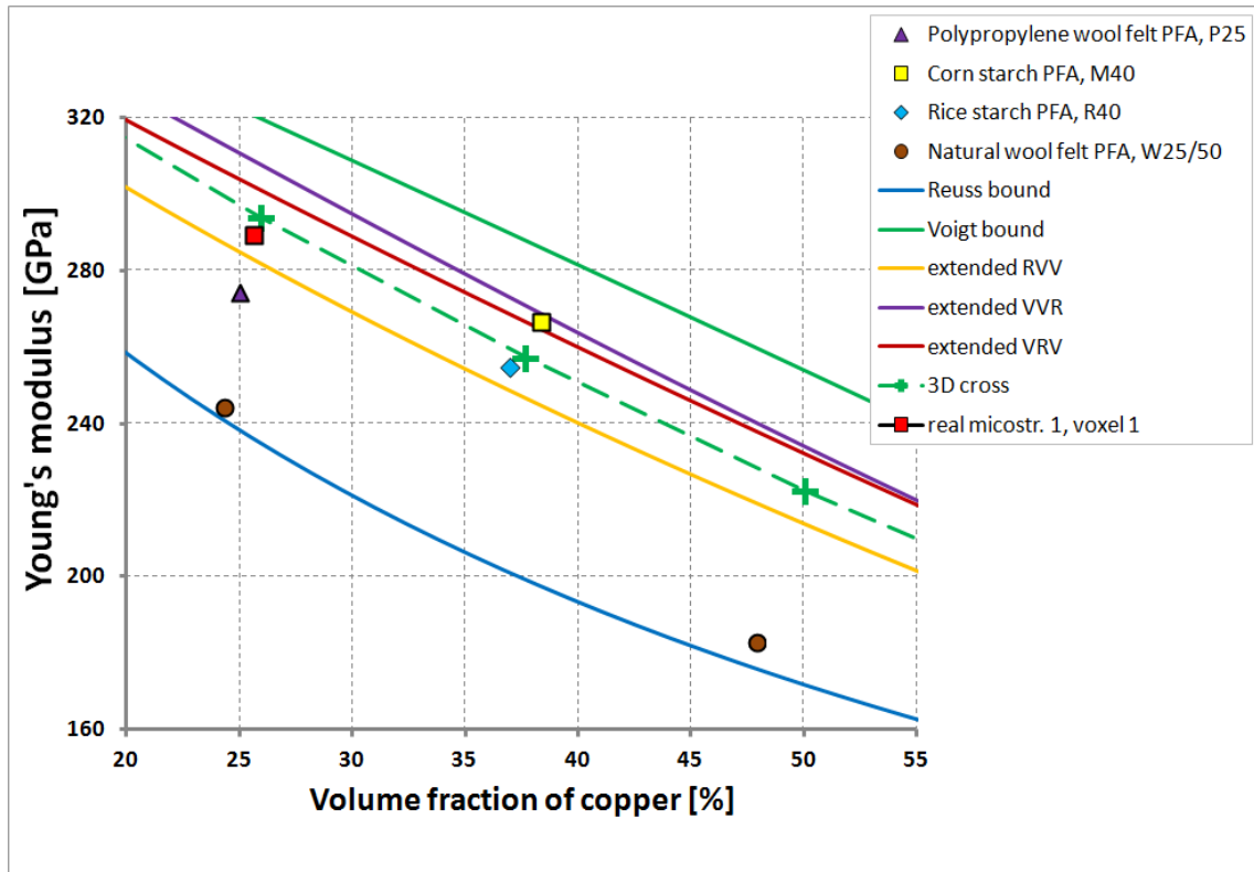
Figure A8. Effect of microstructure and copper content on \text{Al}_2\text{O}_3/\text{Cu} composites Young's moduli. Measurements done with Grindosonic impulse excitation of vibration equipment and compared with Voigt and Reuss bounds, extended V-V-R , R-V-V and V-R-V models and numerical models of 3D cross and of real microstructure for alumina-copper composites at room temperature.
