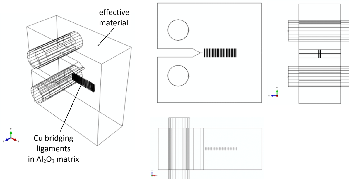
Figure 6.33. Scheme of three-dimensional Compact-Tension model for composite with multiple crack reinforcing parallel fibres, with perspective view and orthogonal projections from ABAQUS
