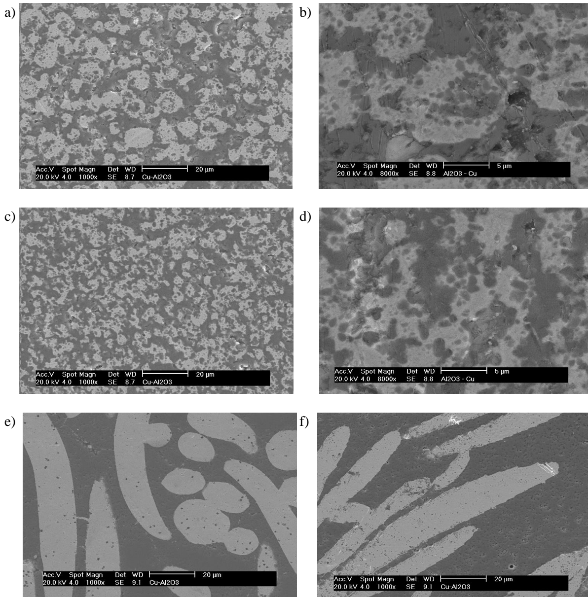
Figure A6. Microstructures of infiltrated \text{Al}_2\text{O}_3/\text{Cu} composites (microscopic images, courtesy of J. Winzer, L. Weiler, J. Rödel, TUD): a) corn starch PFA, 40% Cu (M40), magnification 1000x, b) corn starch PFA, 40% Cu (M40), magnification 8000x, c) rice starch PFA, 40% Cu (R40), magnification 1000x, d) rice starch PFA, 40% Cu (R40), magnification 8000x, e) polypropylene wool felt PFA, 45% Cu, magnification 1000x, f) natural wool felt PFA, 30% Cu, magnification 1000x. Light gray – copper, dark gray - alumina
