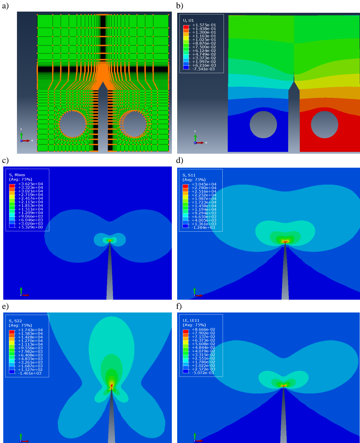
Figure 6.44. (a) Boundary conditions and (b-f) selected results from the global model of the C-T test at applied u_1 = 0.157 mm: (b) displacements in the loading (horizontal) direction u_1 , (c) von Mises stresses in the crack tip vicinity, (d) stresses in the loading (horizontal) direction in the crack tip vicinity, (e) vertical stresses in the crack tip vicinity, (f) logarithmic strains in the loading (horizontal) direction in the crack tip vicinity.
