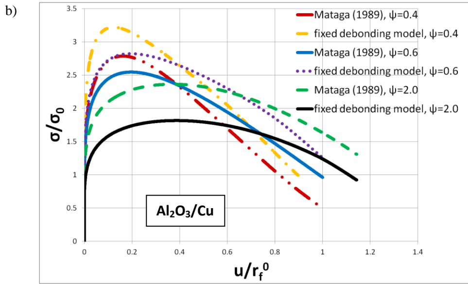
Figure 6.17. Normalized stress-displacement relationships in the reinforcing fibre from the numerical model with fixed debonding lengths, compared with the analytical solutions of Mataga (1989) for different values of debonding parameter \psi : a) Al_2O_3/Al , b) Al_2O_3/Cu .
