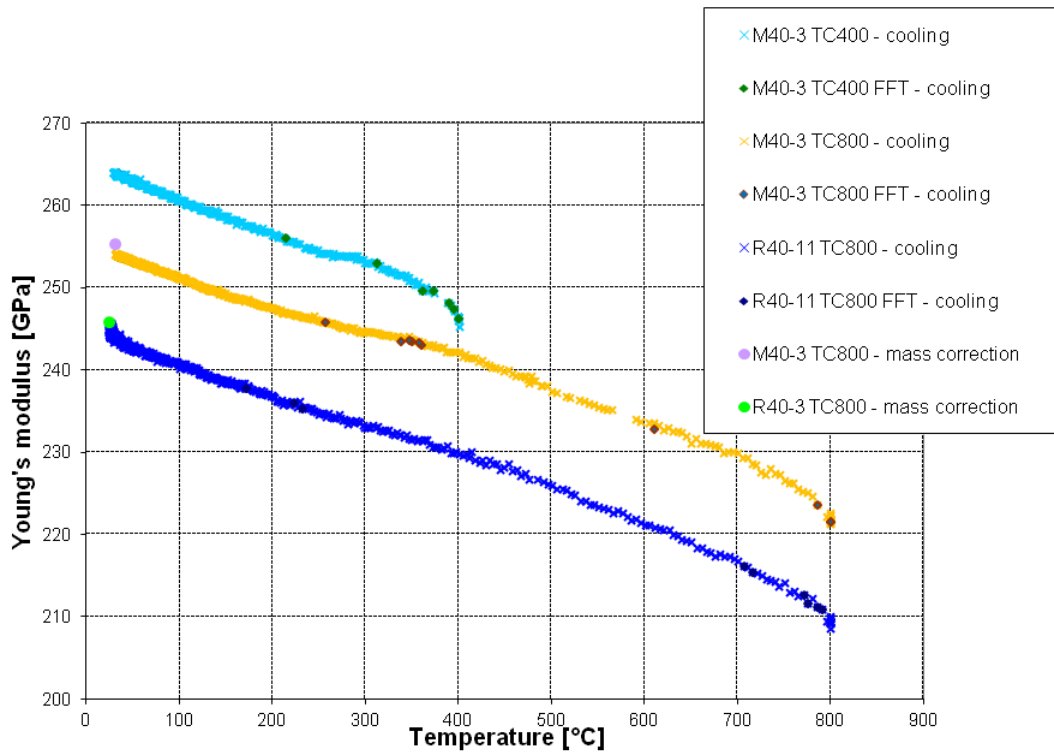
Figure A10. Young's modulus in temperature cycles for Al 2 O 3 /Cu IPCs based on corn and rice starch
