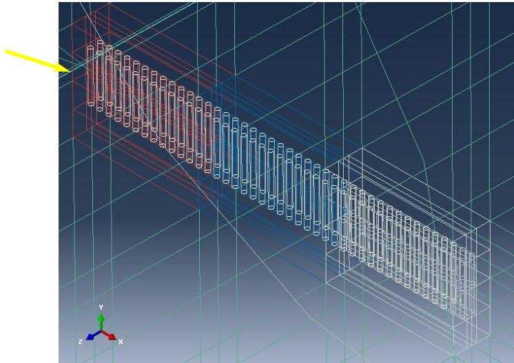
Figure 6.35. Detailed view of the crack tip neighbourhood with family of parallel reinforcing fibres.
