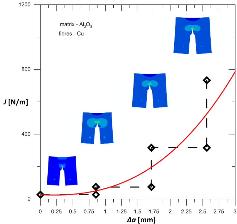
Figure 6.32. Illustrative example of J -integral vs. crack length increase \Delta a curve for plane strain C-T of alumina specimen toughened with copper fibres - results from ABAQUS.
