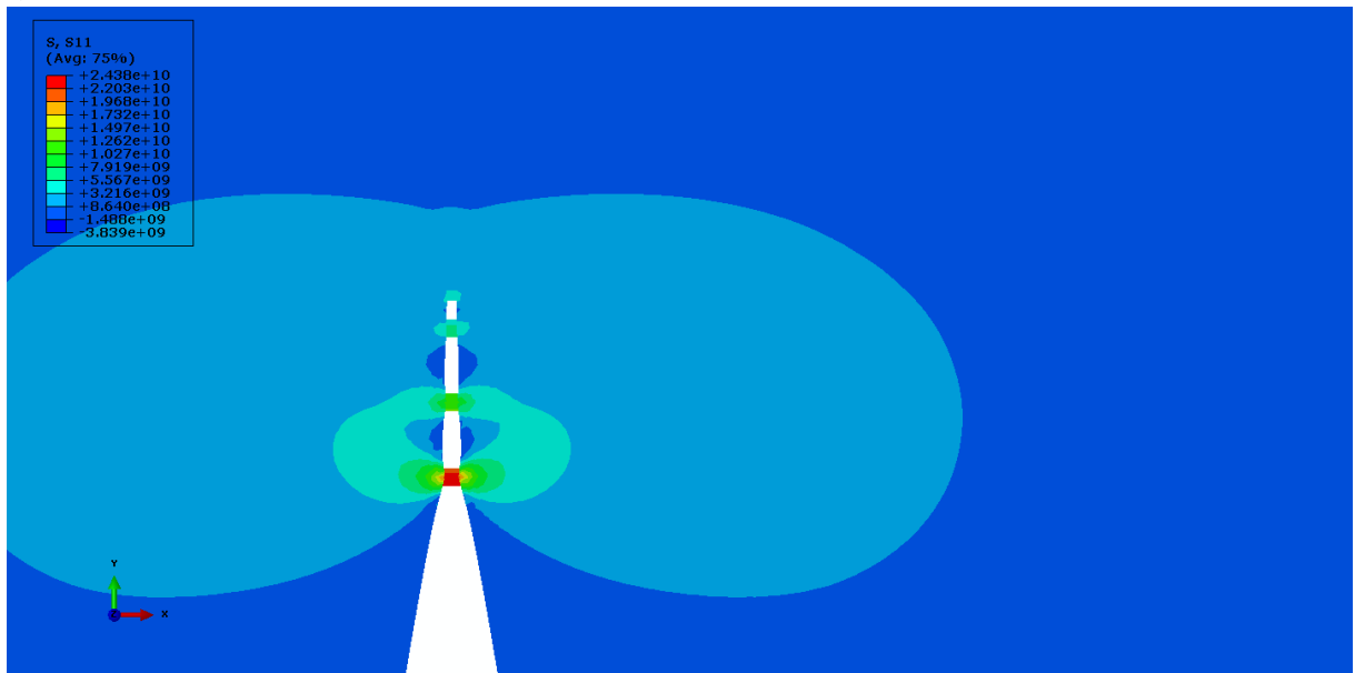
Figure 6.31. Distributions of horizontal stresses for increasing crack length in plane strain C-T model with multiple fibres.
