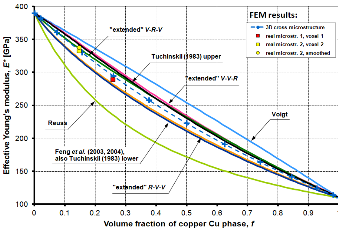
Figure 5.14. Effective Young's modulus of Al_2O_3/Cu IPC in function of copper volume fraction; numerical results for three different microstructures – 3D cross and two real microstructures distinguished with different colours; for one of the real microstructures (yellow marks) two different FEM mesh variants (voxel and smoothed) were used.
