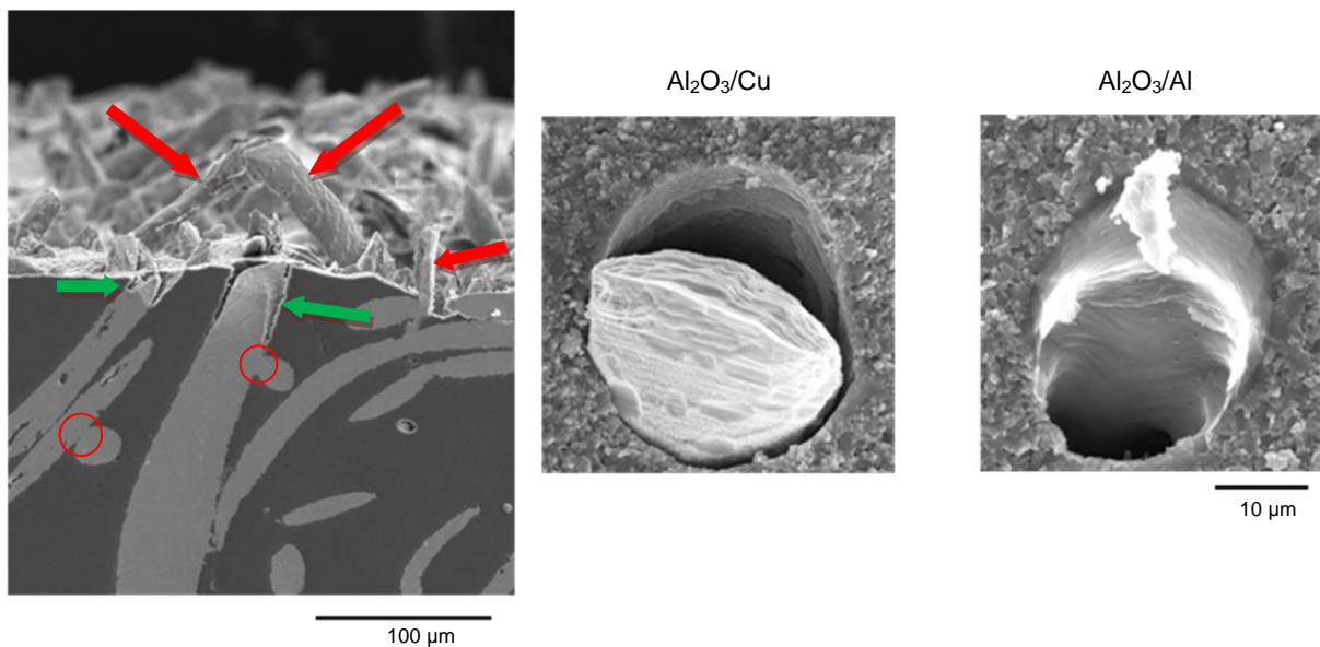
Figure 6.1. Fracture of IPC composites: a) interconnected fibres forming interpenetrating microstructure (connections between fibres marked with circles), different angles between fibres and crack surface (marked with red arrows), and debonding between fibre and matrix (marked with green arrows), b) and c) – different shapes and sizes of debonding on examples of alumina-copper and alumina-aluminum composites (SEM images from reports of KMM-NoE FP6 EU project by L. Weiler, TU Darmstadt and J. Dusza, IMR SAS).
