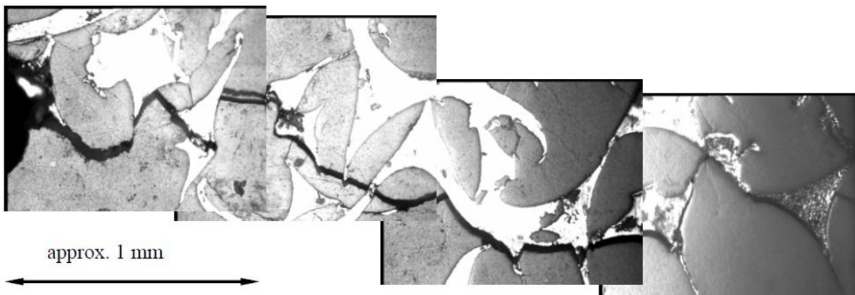
Figure 6.3. Panoramic view of the crack path in Al 2 O 3 /Cu IPC specimen.
