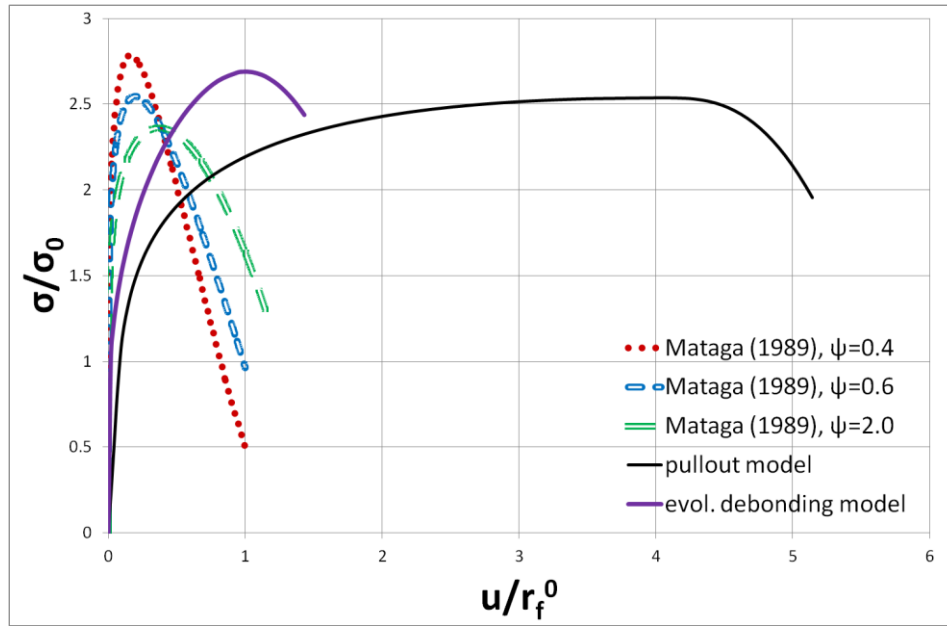
Figure 6.25. Comparison of the stress-displacement relationships in Cu fibre obtained according to the “pullout” and “evolving debonding” models with (a) fixed debonding model, and (b) Mataga model (for different values of \psi ).
