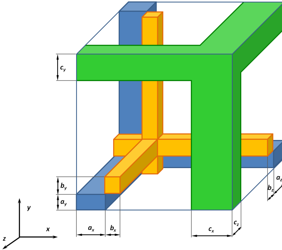
Figure 2.2 The Feng et al. (2003, 2004) unit cell of an interpenetrating four-phase composite with phases that have different dimensions in each direction x , y , z ; blue a , yellow b and green c phases visible, fourth phase invisible (based on Feng et al. (2003, 2004), with the permission of publishers).
