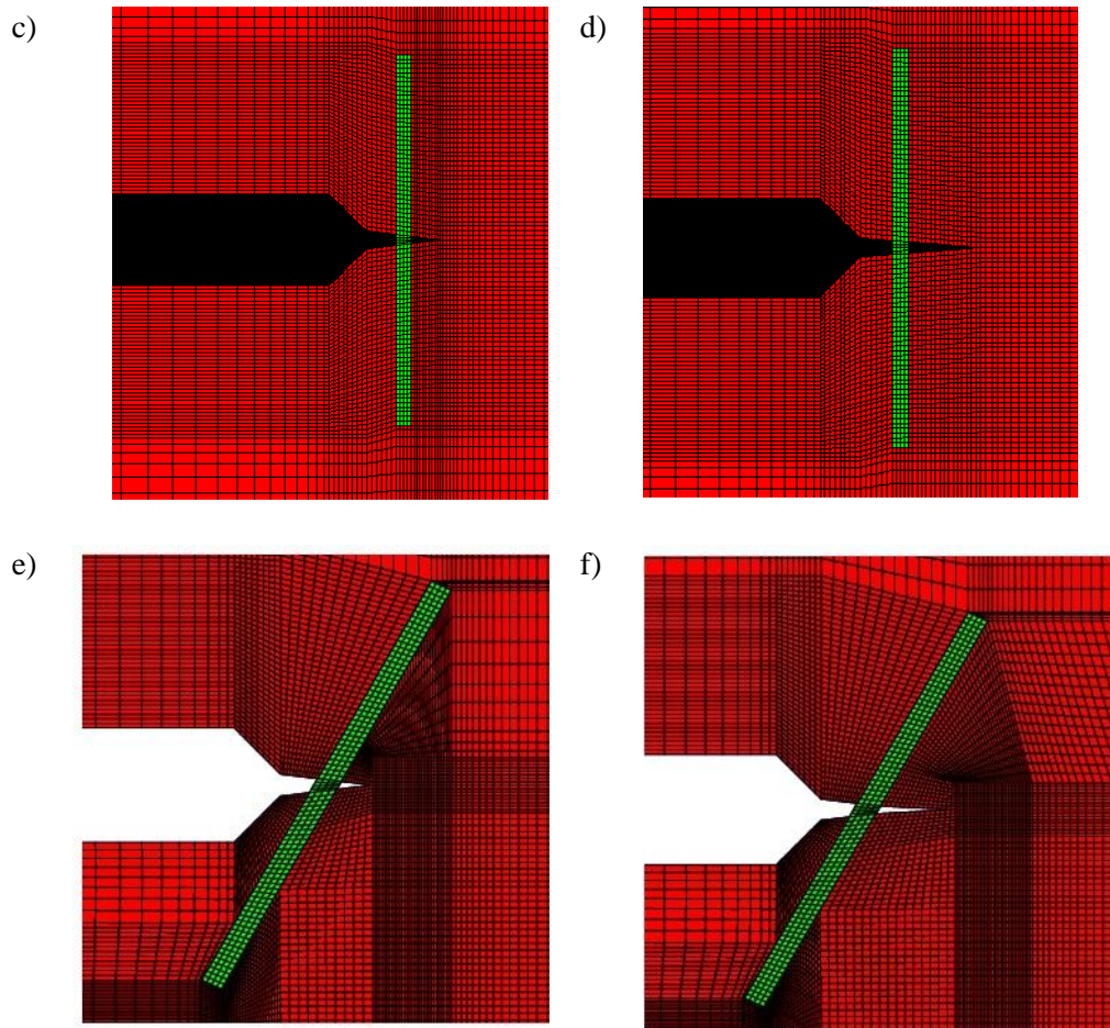
Figure 6.27. Pre-cracked C-T specimen model in FEAP – FE mesh in the vicinity of the crack tip (red colour – ceramic, green colour – metal): (a), (b) monolithic ceramics; (c), (d) with reinforcement inclined 90^\circ to the crack plane; (e), (f) with reinforcement inclined 60^\circ to the crack plane; (a), (c), (e) – before, and (b), (d), (f) – after the crack length increase (images are not in the same scale).
