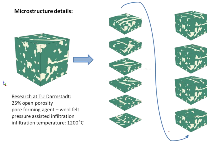
Figure 6.40. Details of the microstructure of real IPC cube - horizontal cuts through the piece from bottom to top, with visible bridging ligaments and interconnections between fibres.
