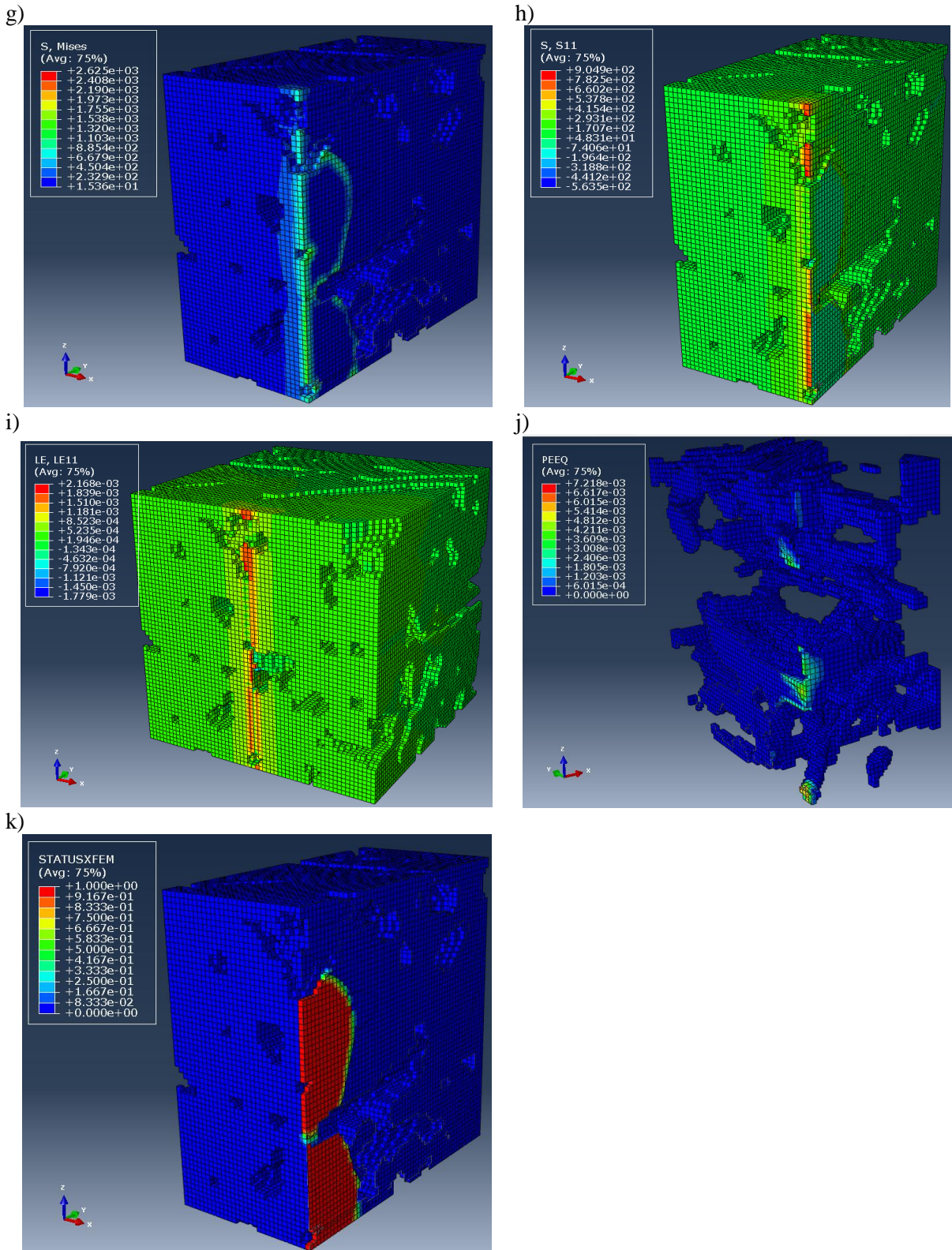
Figure 6.45. Selected model results obtained for the real IPC piece: (a) propagated crack marked with red (white – copper phase), (b) displacements in the loading direction in the copper phase, (c-g) von Mises stresses, (d-f) - in the copper phase, (e) – left half, (f) – right half, (g) –left half of the ceramic phase, (h) stresses in the loading direction in the ceramic phase, (i) logarithmic strains in the loading direction in the ceramic phase, (j) plastic equivalent strains in the copper phase (right half), (k) propagated crack marked with red in the ceramic phase (left half).
