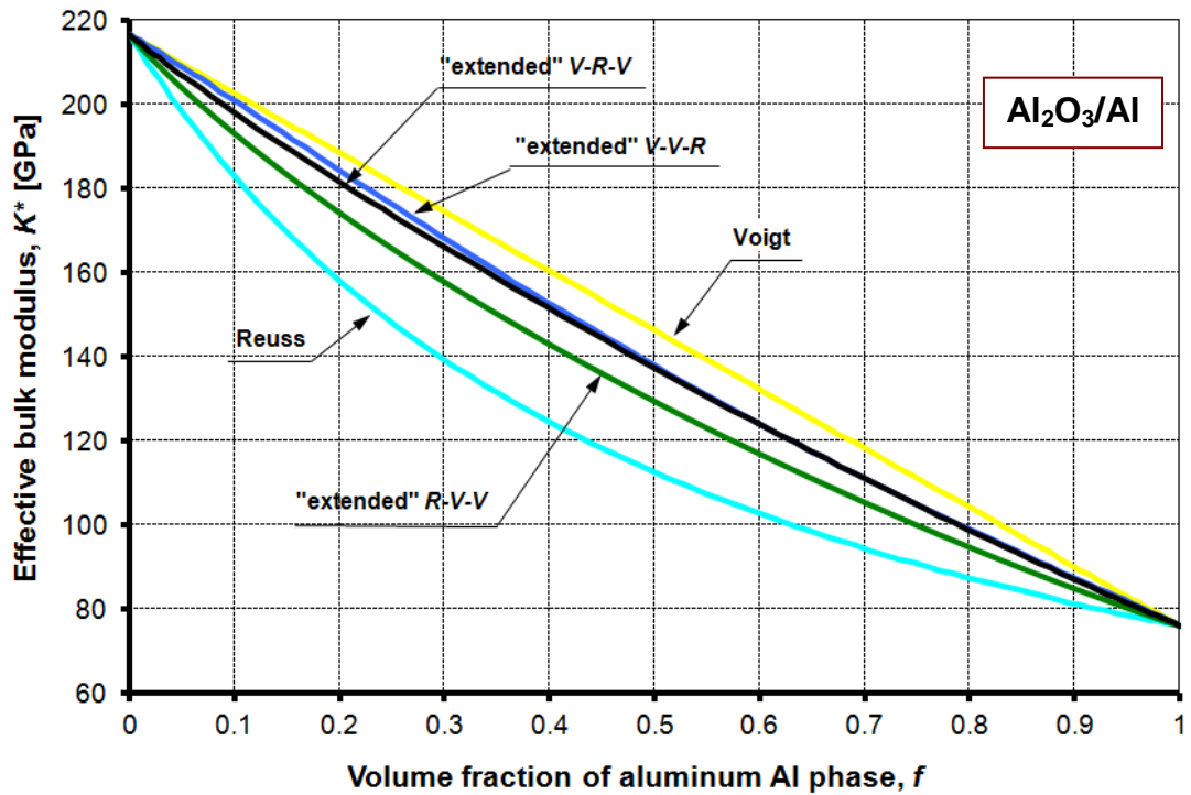
Figure 5.5. Effective bulk moduli vs. volume fractions of metal phase.
