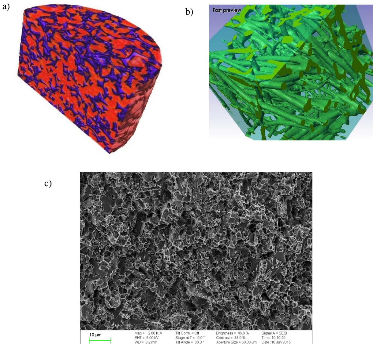
Figure 1.1. Examples of metal-ceramic composite materials with interpenetrating microstructure (IPCs): a) Al 2 O 3 /Cu composite, red colour - alumina phase, blue - copper phase (courtesy of G. Geier, Leoben), b) image of copper phase in Al 2 O 3 /Cu composite obtained with Simpleware ScanIP software, c) SEM image of fracture surface of Al 2 O 3 preform of 34% open porosity pressure infiltrated with Al alloy 44200 (courtesy of PZMK IPPT PAN).
