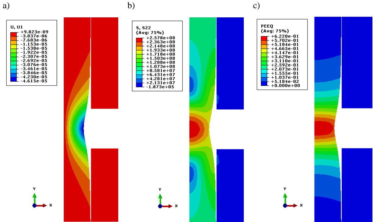
Figure 6.23. Distributions of radial displacements (a), axial stresses (b), and equivalent plastic strains \bar{\epsilon} (c) at axial displacement u_2 = 0.25\text{mm} .
