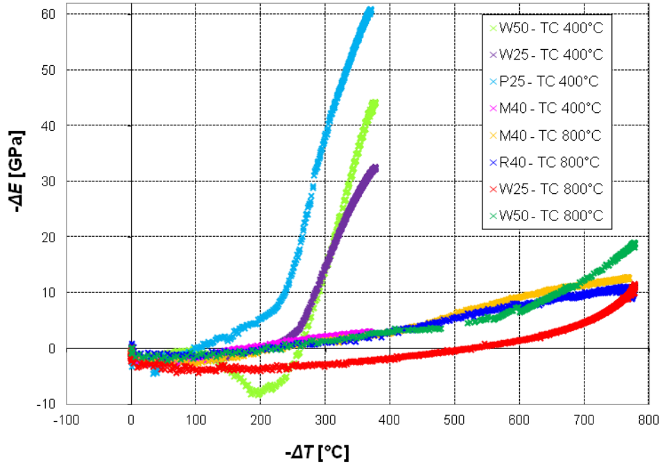
Figure A11. Reduction of Young's modulus vs. temperature decrease in cooling, temperature cycles up to 400°C and 800°C for Al 2 O 3 /Cu IPC composites with different microstructures and copper contents (the idea of the graph is explained in Figure A9).
