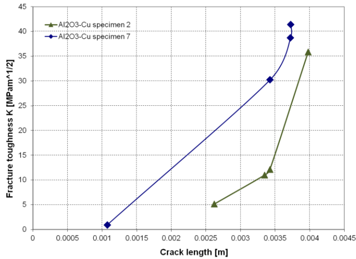
Figure 6.5. Experimental measurements of fracture toughness of Al 2 O 3 /Cu IPC in four-point bending as a function of crack length ( R-curves ).
