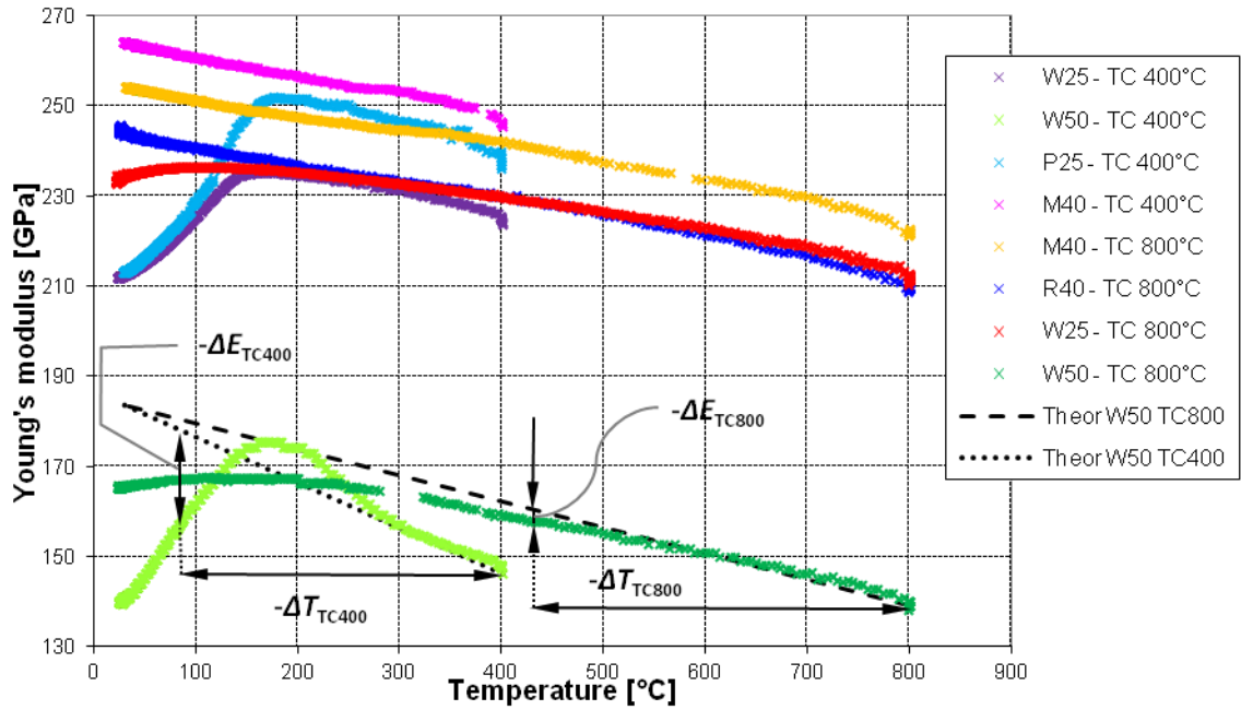
Figure A9. Young's moduli in temperature cycles RT-400°C and RT-800°C for Al 2 O 3 /Cu composites with different microstructures and copper contents. On the example of W50 IPC specimen, the idea of Galal-Yousef (2004; 2005) is presented how to obtain curves showing differences between theoretical and real Young's moduli decrease upon cooling for two thermal cycles RT- 400°C and RT-800°C.
