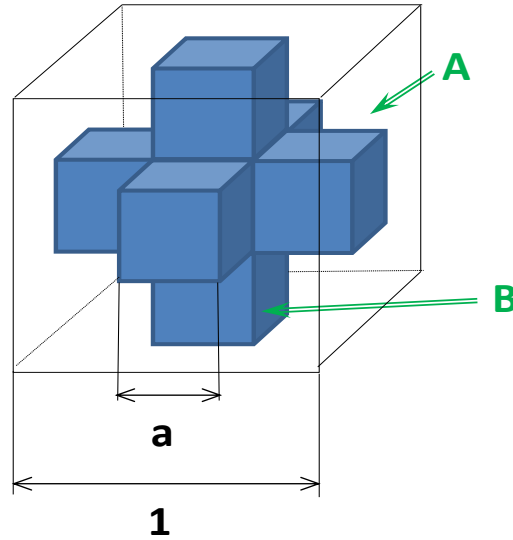
Figure 2.1. Unit cell representing two-phase interpenetrating microstructure, according to Frey (1932) and Tuchinskii (1983).
