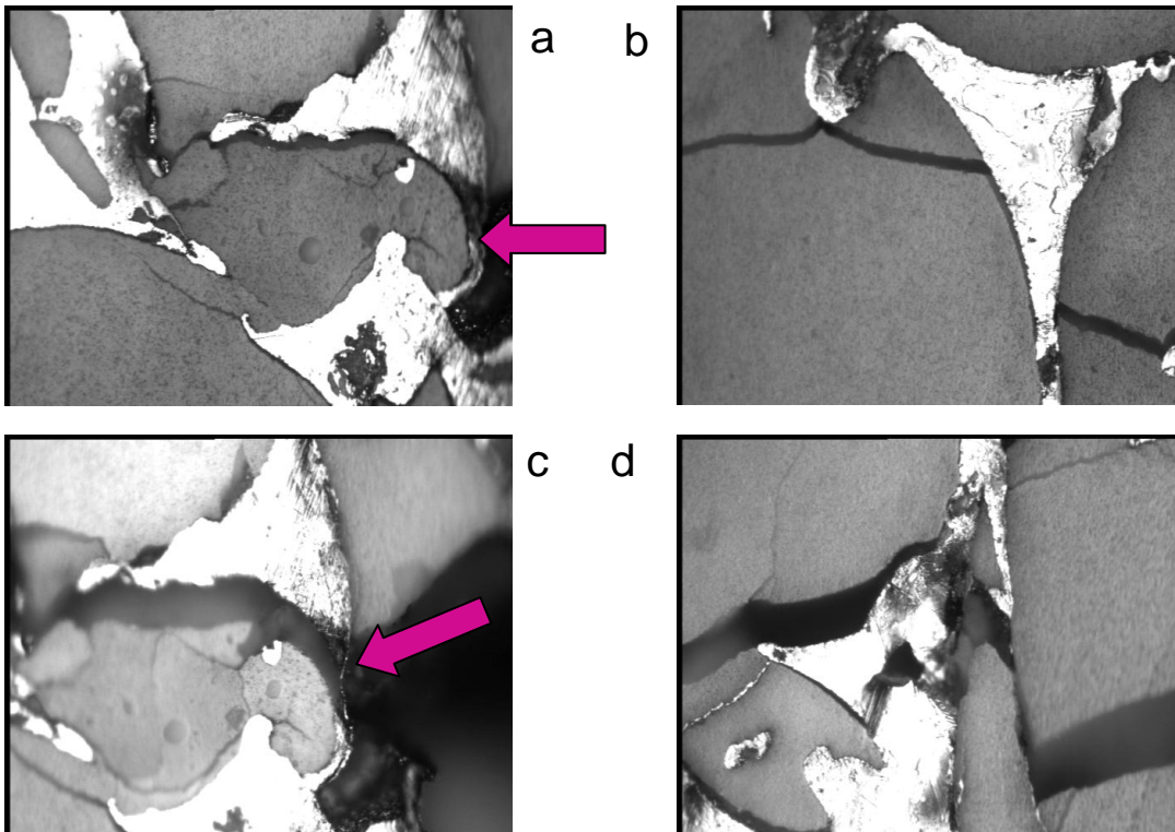
Figure 6.2. Crack development in Al 2 O 3 /Cu IPC specimen: a) initial load (~40 N), notch end area with widening debonding (arrow indicates a copper bridge that hinders crack growth), b) crack developing along interfaces in the middle of the specimen (load ~100 N), c) notch end area with copper ligament that just has broken (indicated by arrow) with visible large plastic deformation, d) middle of the specimen with strong crack bridging
