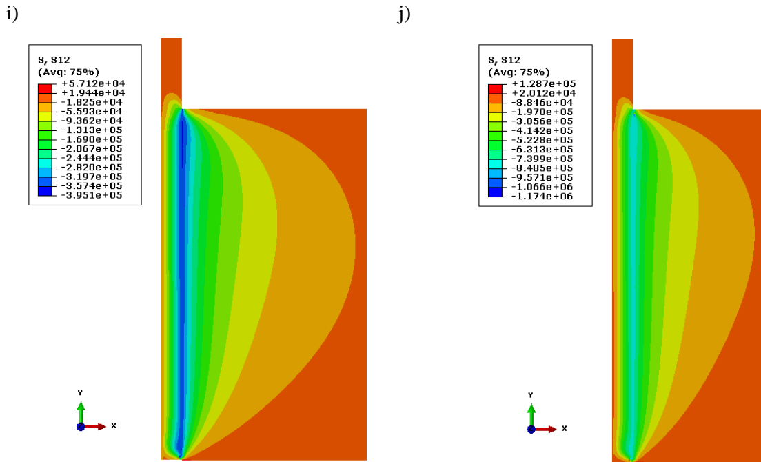
Figure 6.19. (a) – (f): Distributions of von Mises stresses at pullout stages for Cu/Al 2 O 3 : a) elastic deformation of the fibre, b) after initiation of yielding, c) thinning of the fibre visible on the entire pulled out length, d) maximum stresses start to localize, e-f) neck formation; g) Radial displacements u_1 distributed in the pulled out fibre; h) Axial stresses \sigma_{22} in the necking zone; (i) –(j): Distributions of shear stresses \tau_{12} : (i) before initiation of the interfacial crack, (j) after initiation of the interfacial crack. The debonding shear stress in the interface \tau_{\max,0} = 10.0 MPa.
