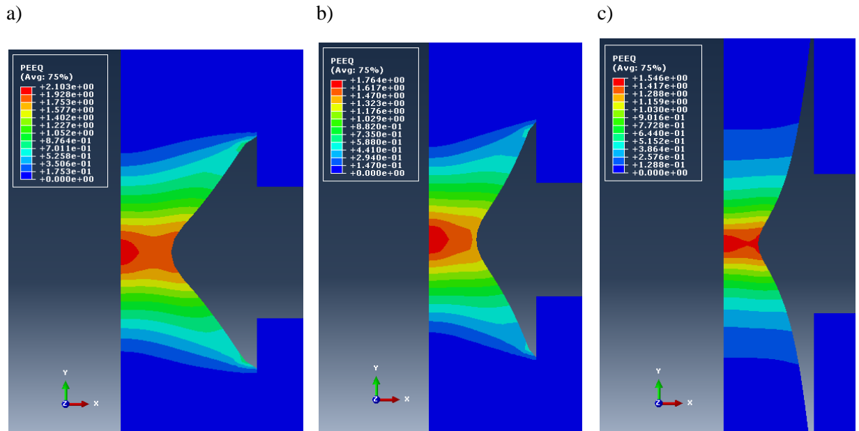
Figure 6.16. Axisymmetric model of uniaxial tension of cracked elastic matrix with reinforcing elastic-plastic fibre at fixed debonding lengths. Distributions of equivalent plastic strains \varepsilon_{pl}^{EQ} (for different loadings u_2 ), for \text{Al}_2\text{O}_3/\text{Cu} : (a) \psi=0.4 , u_2=0.16 mm, (b) \psi=0.6 , u_2=0.175 mm, (c), \psi=2.0 , u_2=0.2 mm (images not in the same scale).
