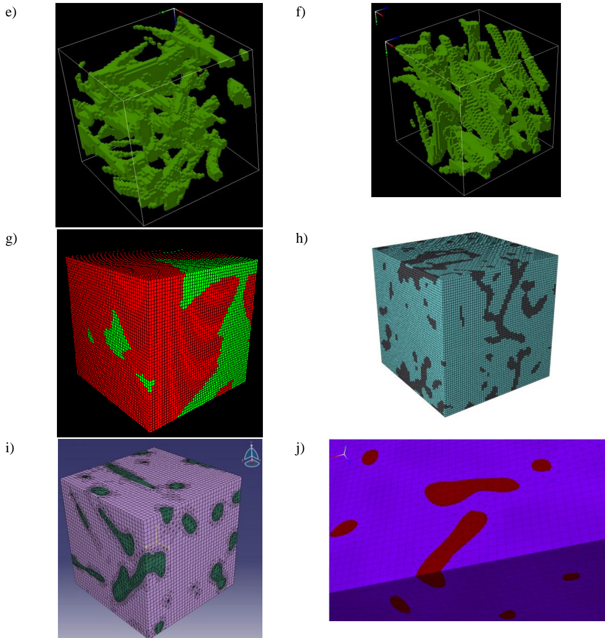
Figure 5.12 Microstructure images obtained with Simpleware ScanIP programme: (a-f), FE meshes used for calculations (g-j), (e-h) - voxel meshes, (i, j) - smoothed meshes: g) microstructure “1”, image created with FEAP 7.5, (h, i) microstructure “2” image created with ABAQUS 6.10, j) mesh created with Simpleware ScanIP/FE. Figures a), b) and i) reprinted with permission of Advanced Engineering Materials.
