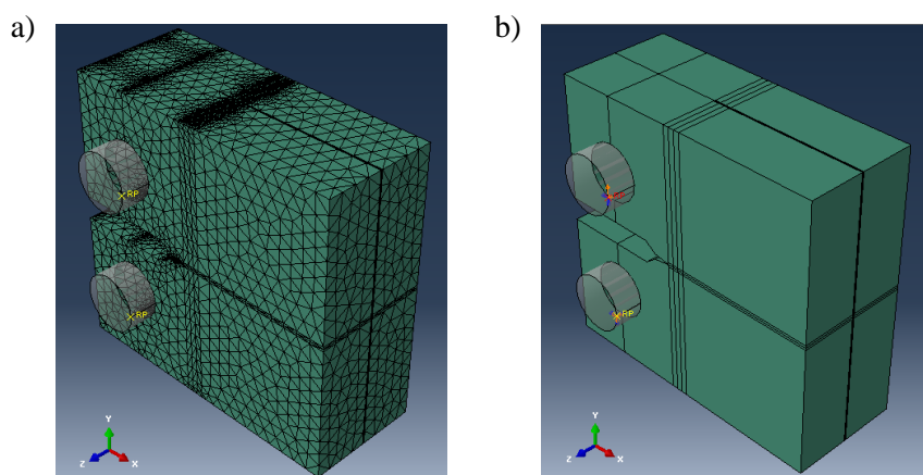
Figure 6.34. Simplified 3D model of Compact-Tension test with parallel fibres near the crack tip: a) sample FE mesh, b) boundary conditions
