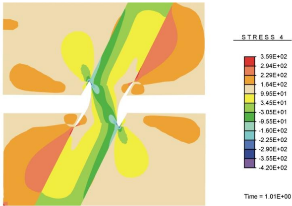
Figure 6.10. a) FEM mesh and boundary conditions, b) materials: red - \text{Al}_2\text{O}_3 , green - Cu, c-e) stress distributions for nondimensional debonding parameter \psi = 1.0 : normal - horizontal (c), normal -vertical (d), and shear (e)
