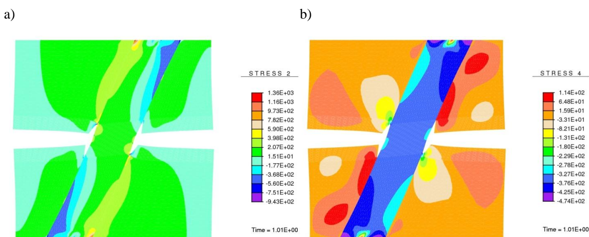
Figure 6.12. Stress distributions for elastic fibre in elastic-plastic matrix: a) normal stress in vertical direction b) shear
