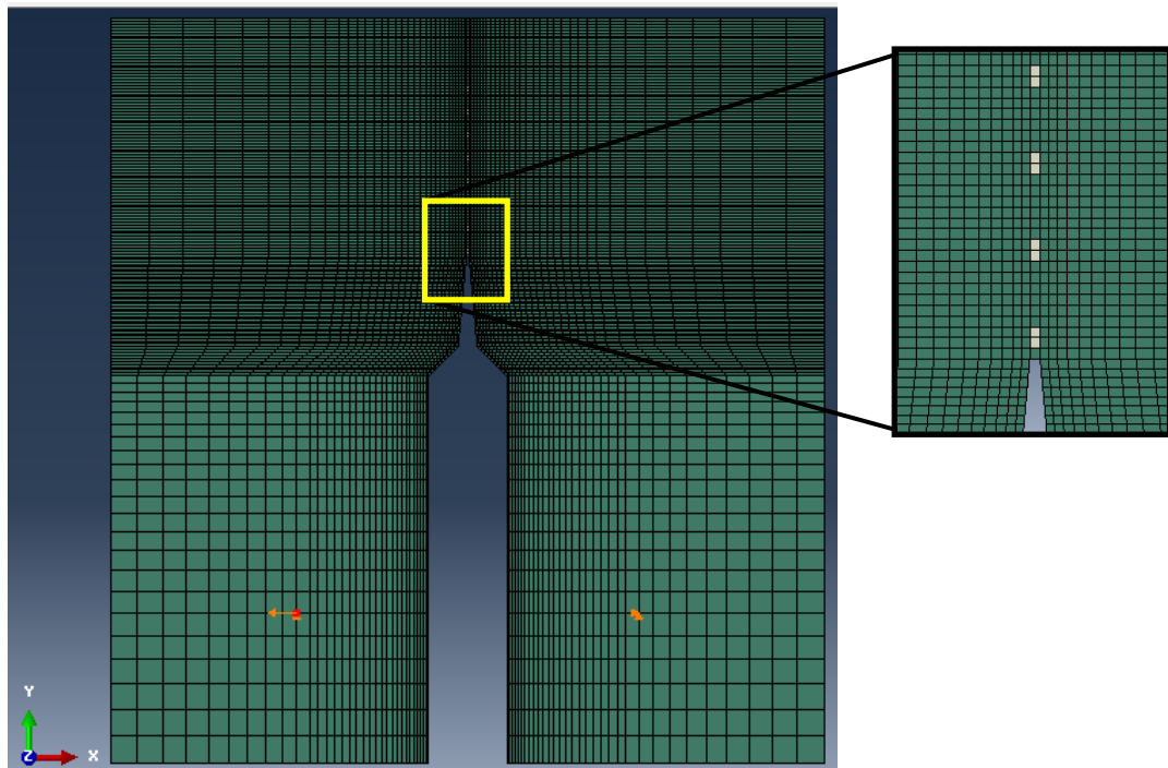
Figure 6.30. Compact-Tension (C-T) test model in ABAQUS (mesh created with FEAP) with bridging fibres modelled as plane strain elements (light colour), boundary conditions and displacement loading
