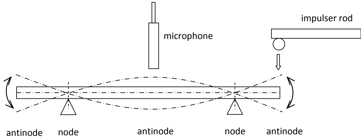
Figure A7. Detection of fundamental flexural resonant frequency of a vibrating specimen
