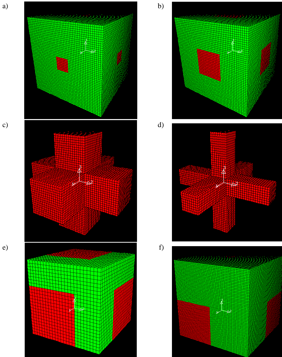
Figure 5.9. FEM model of the cubic unit cell created with FEAP 7.5 for different metal volume fractions; red phase – alumina, green phase – copper. (a, b) Unit cell model used for the calculations of the effective Young’s modulus and Poisson’s ratio, (c, d) – one of the phases with another phase invisible, (e, f) 1/8^{\text{th}} of the unit cell used for the effective shear modulus calculations. Volume fractions of metal: a), d) 0.93, b), c) 0.74, e) 0.26, f) 0.50, finer mesh.
