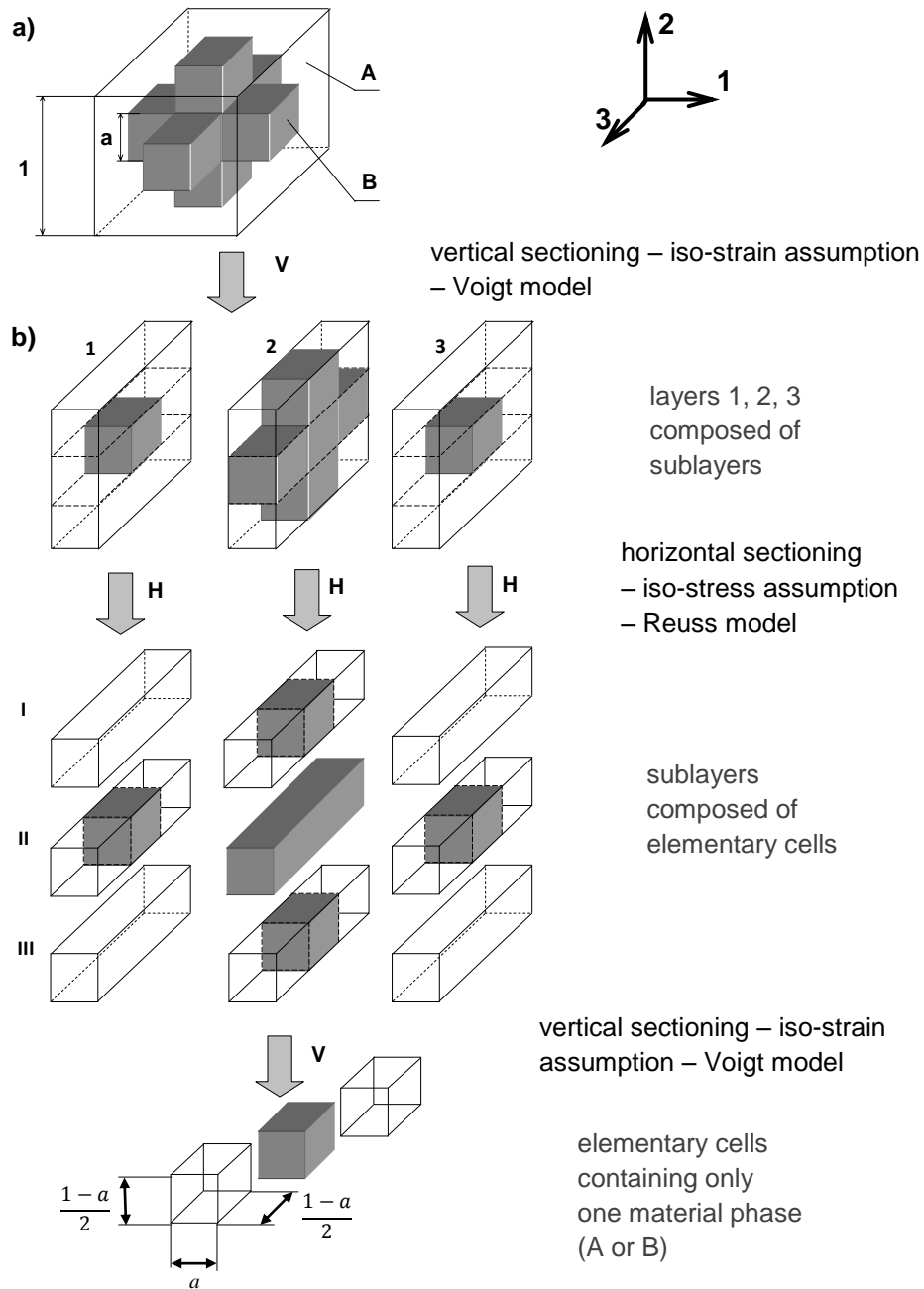
Figure 5.1. (a) Unit cell of a simplified interpenetrating microstructure (“cross microstructure”) based on the models of Frey (1932), Turchinskii (1983) and Feng et al. (2003, 2004), used in modelling of effective mechanical properties of IPCs, (b) decomposition sequence of the unit cell according to the “extended” V-R-V model in vertical (V) and horizontal (H) directions (reprinted with permission of Computational Materials Science ).
