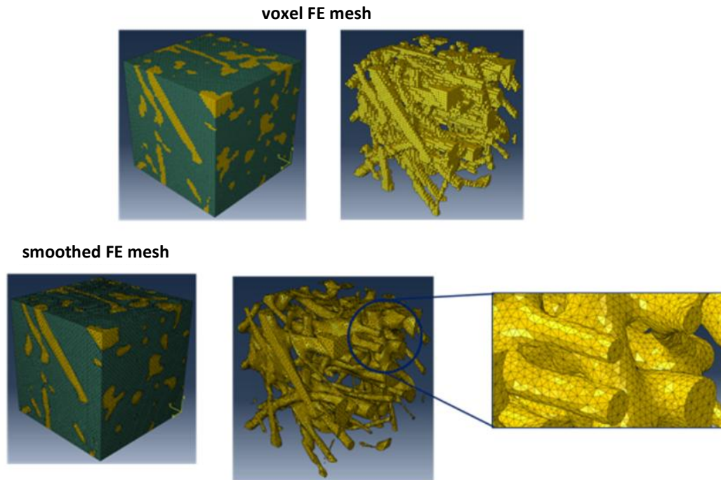
Figure 5.13 Effect of mesh smoothing microstructure images obtained with ABAQUS 6.10.
