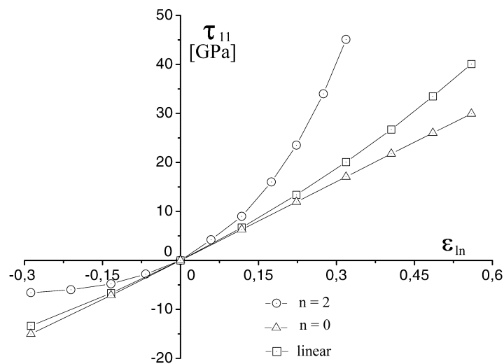
Fig. 5. Kirchhoff stress – logarithmic strain diagram for uniaxial strain
