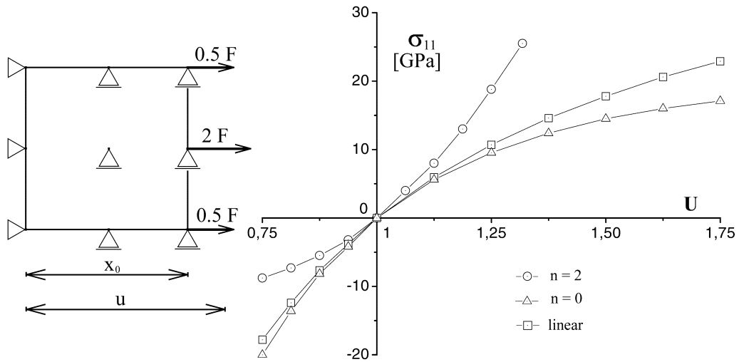
Fig. 4. Layout and response diagram for uniaxial strain
