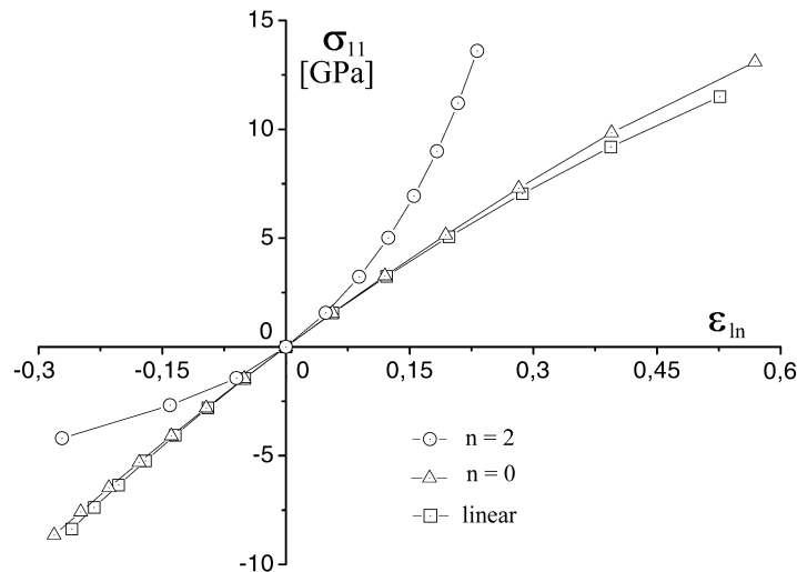
Fig. 3. Kirchhoff stress – logarithmic strain diagram for uniaxial stress
